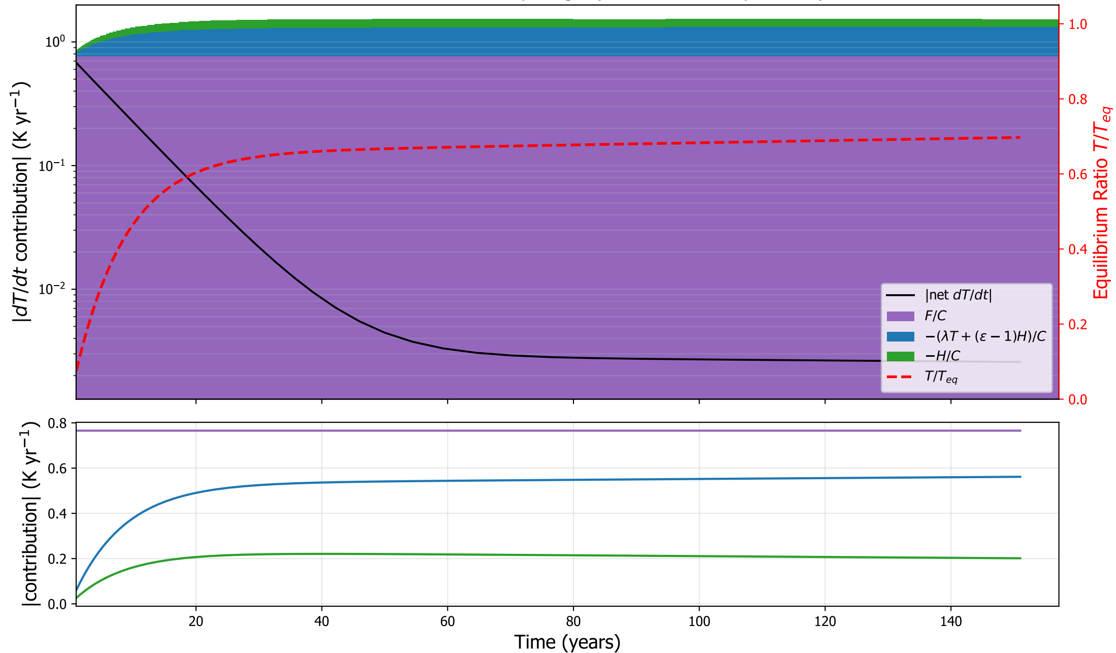
HadGEM2: surface tendency budget ( \varepsilon=1.14 , \tau_s=1112 yr, C=7.9 )
