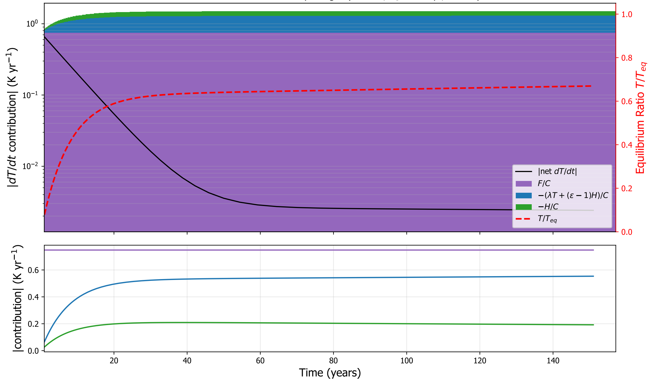
IPSLCM5A: surface tendency budget ( \varepsilon=1.27 , \tau_s=1223 yr, C=8.6 )
