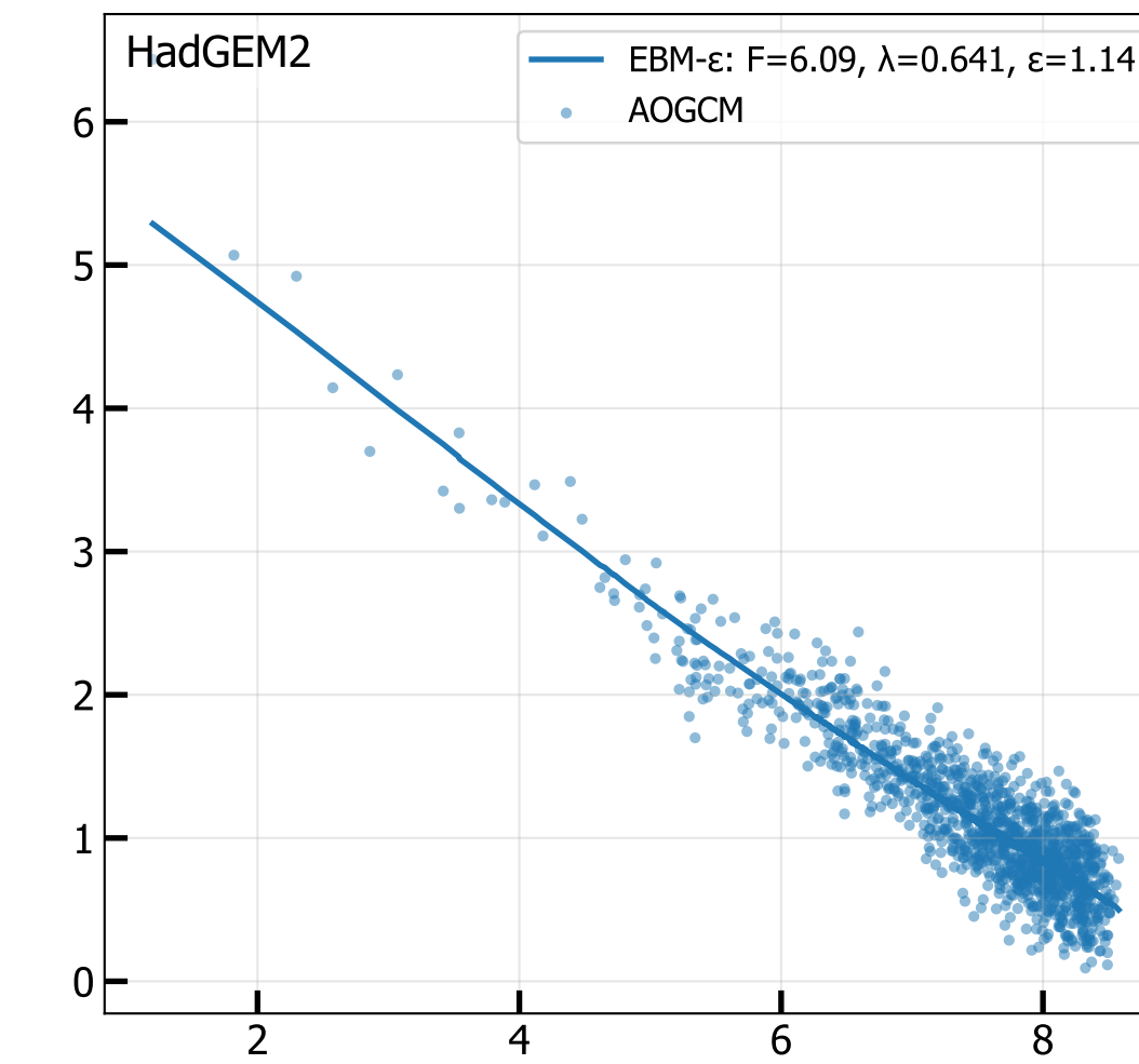
2-meter Air Temperature Anomaly (K)
