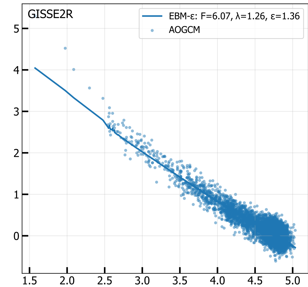
Net TOA Radiative Flux Anomaly ( W m^{-2} )
