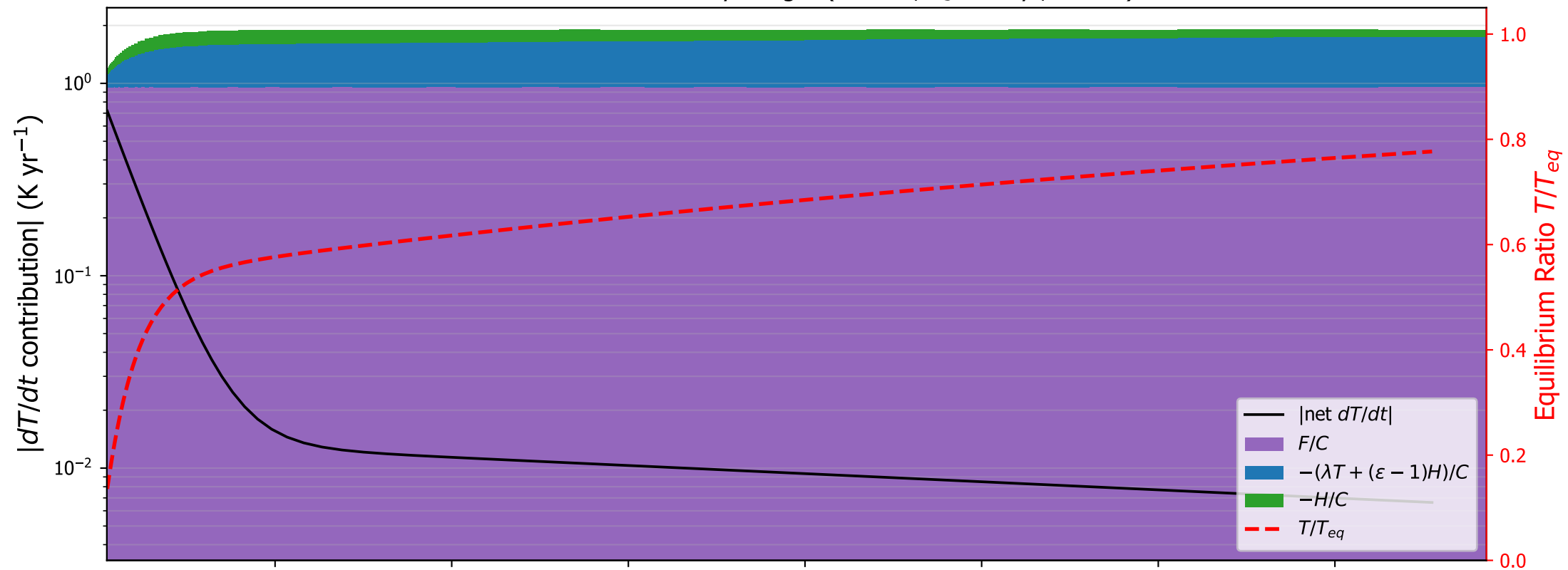
CESM1: surface tendency budget ( \varepsilon=1.35 , \tau_s=206 yr, C=8.0 )
