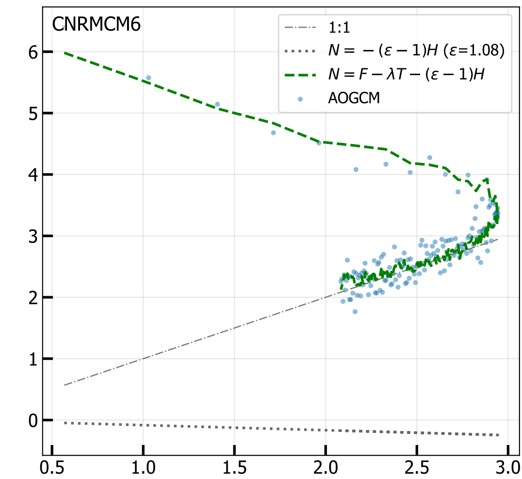
4xCO 2 Net TOA vs Ocean Heat Uptake H (radiative fit, iter 2)
