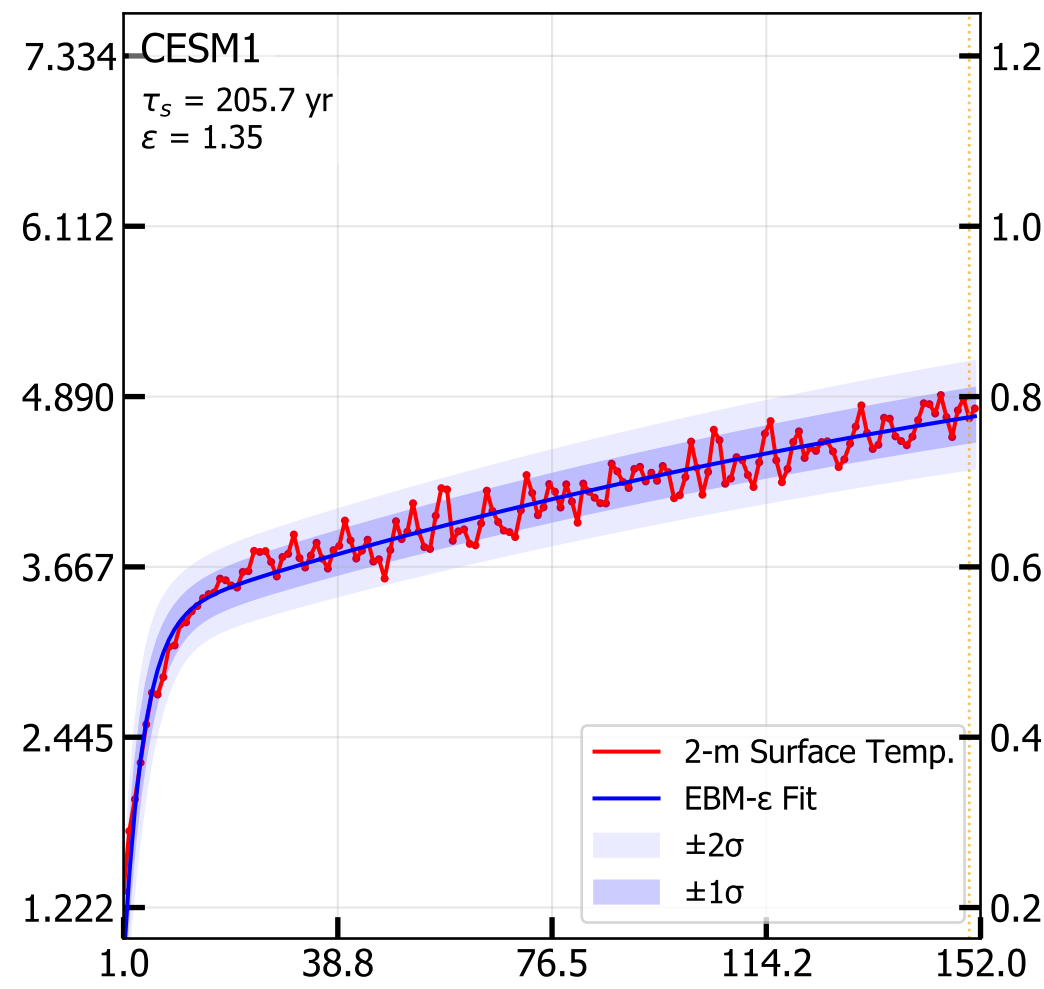
4xCO 2 T 2M vs. Time w/ EBM-ε Fit
