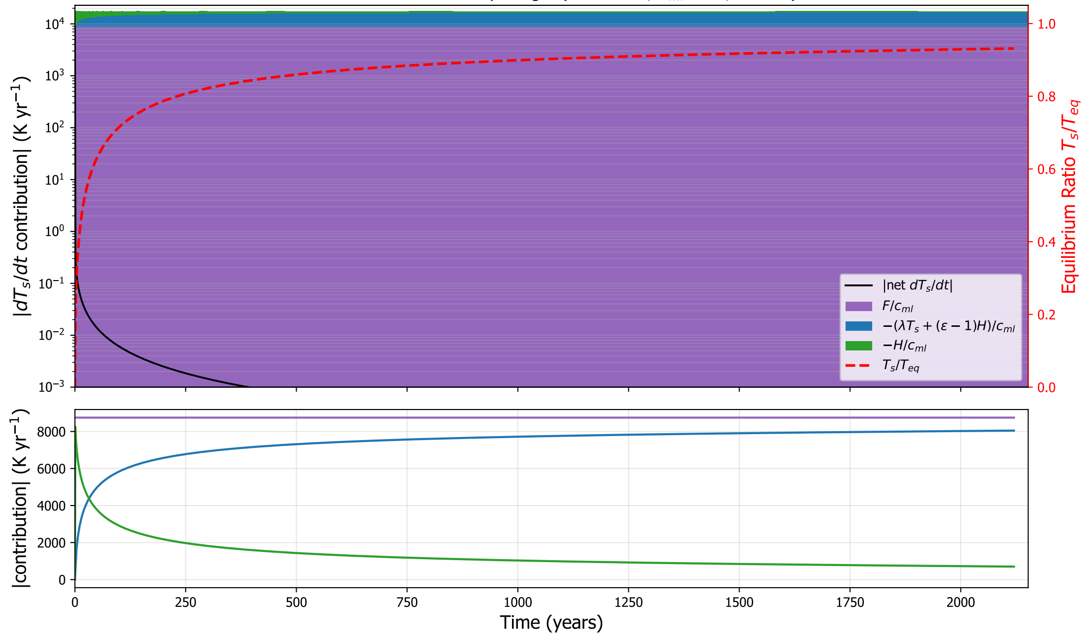
CCSM3: surface tendency budget ( \kappa=5.6\text{e-}05 , h_{ml}=0 m, \varepsilon=0.86 )
