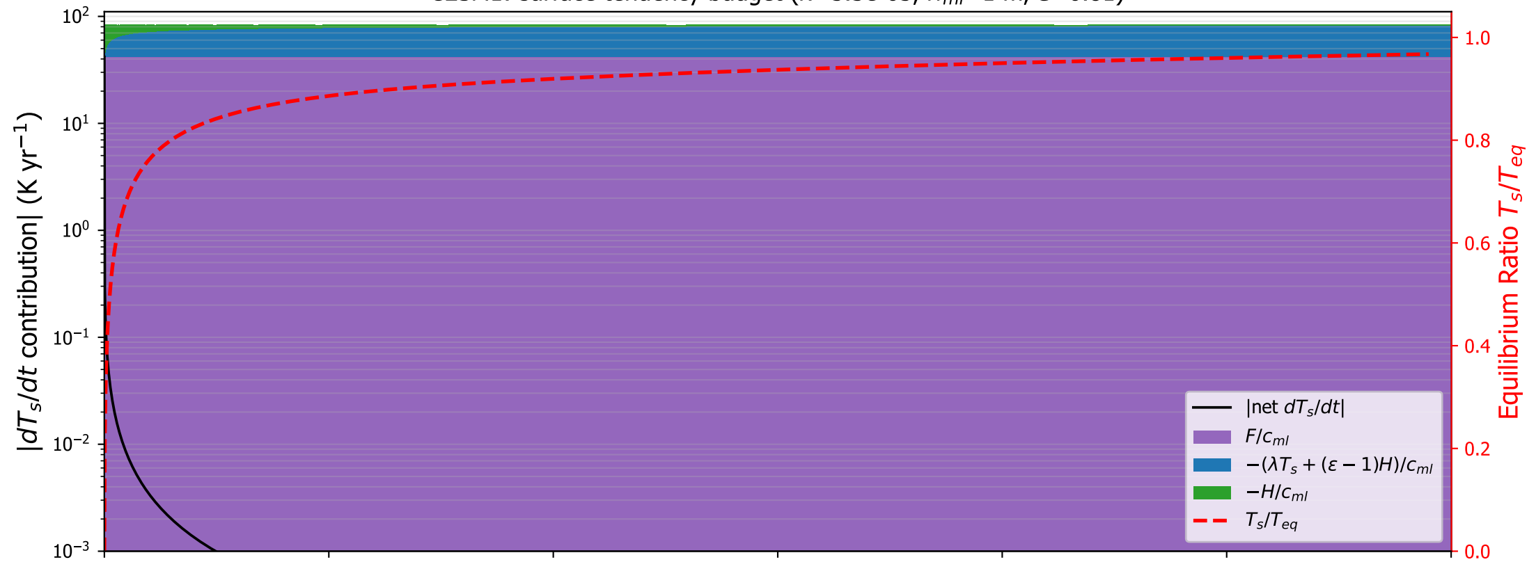
CESM1: surface tendency budget ( \kappa=5.3\text{e-}05 , h_{ml}=1 m, \varepsilon=0.81 )
