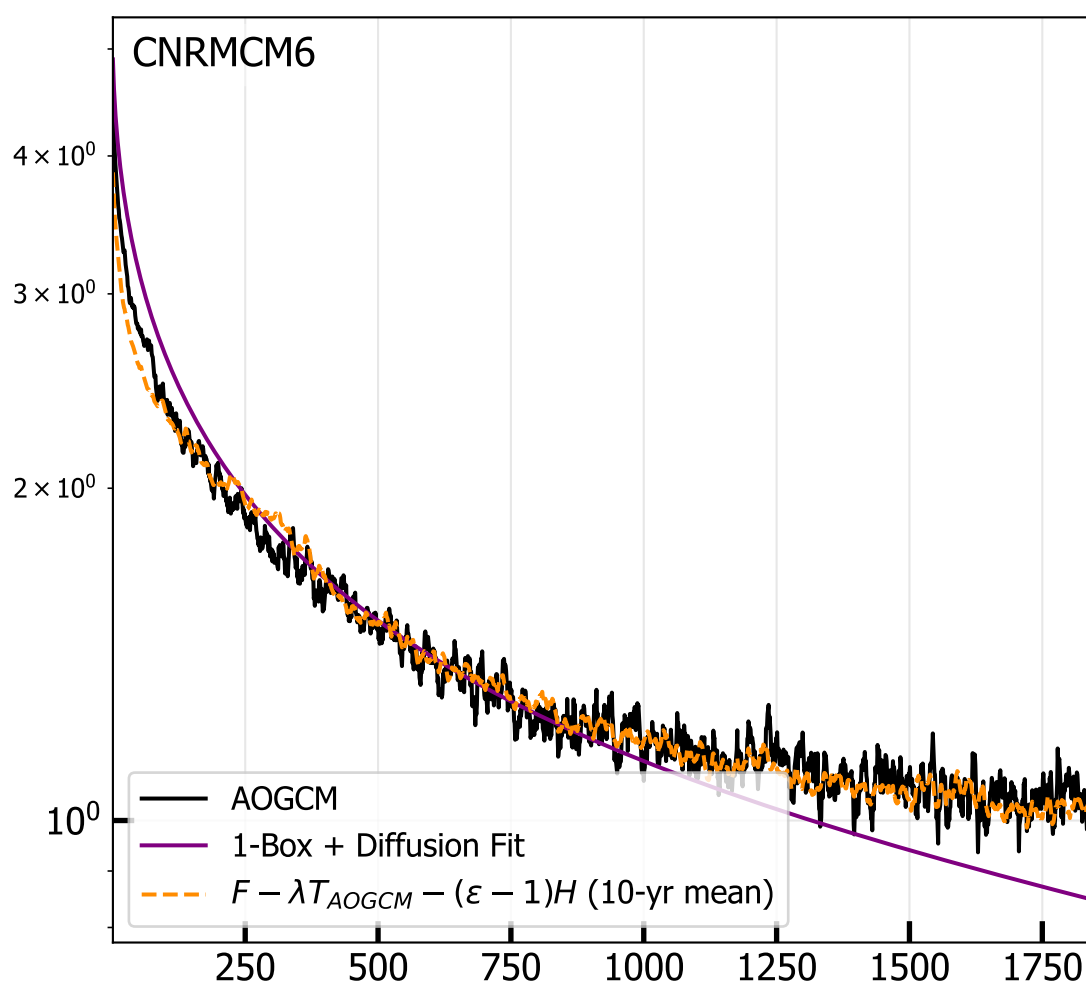
4xCO 2 Net TOA vs. Time
