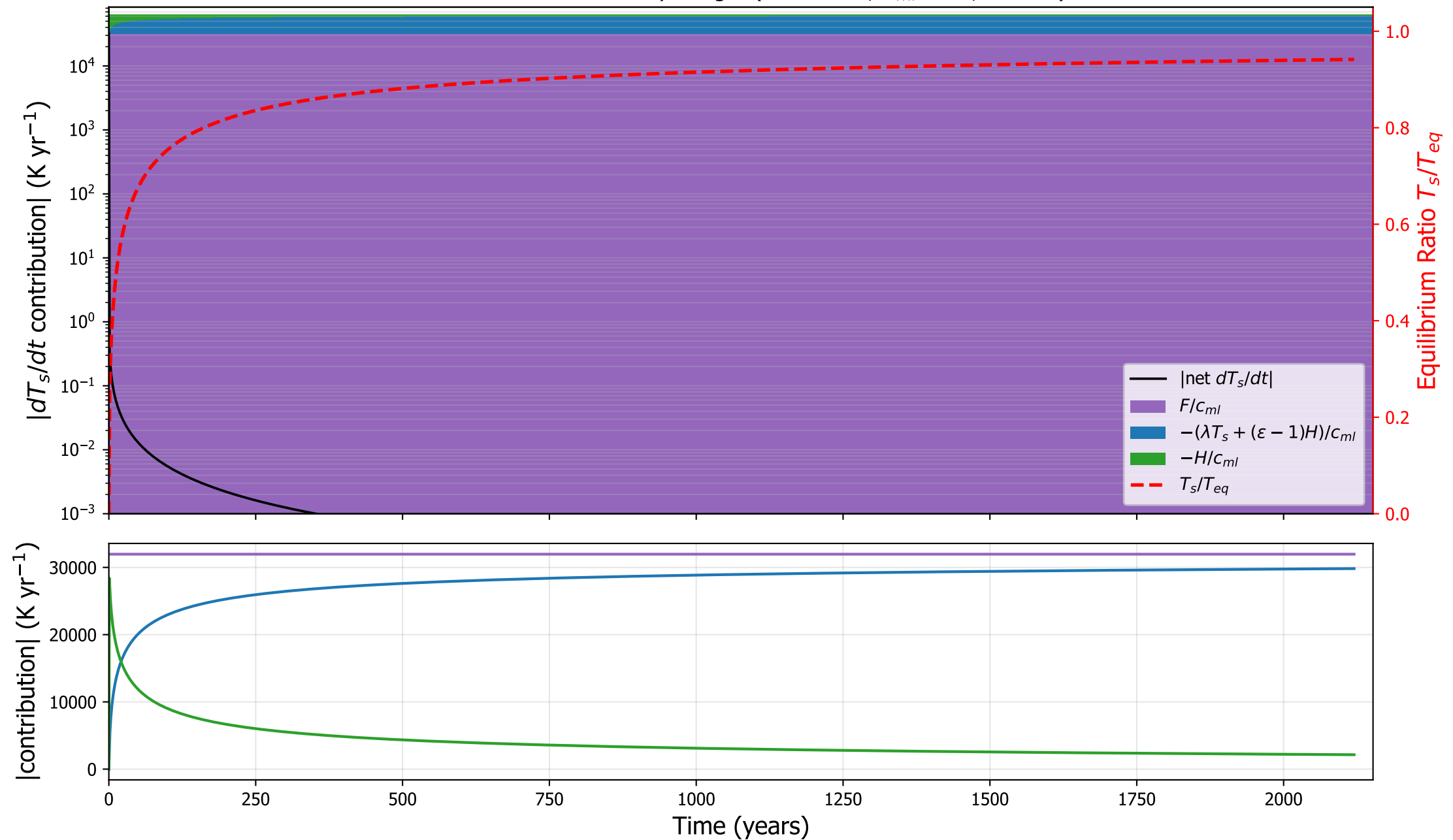
CCSM3: surface tendency budget ( \kappa=4.1\text{e-}05 , h_{ml}=0 m, \varepsilon=0.87 )
