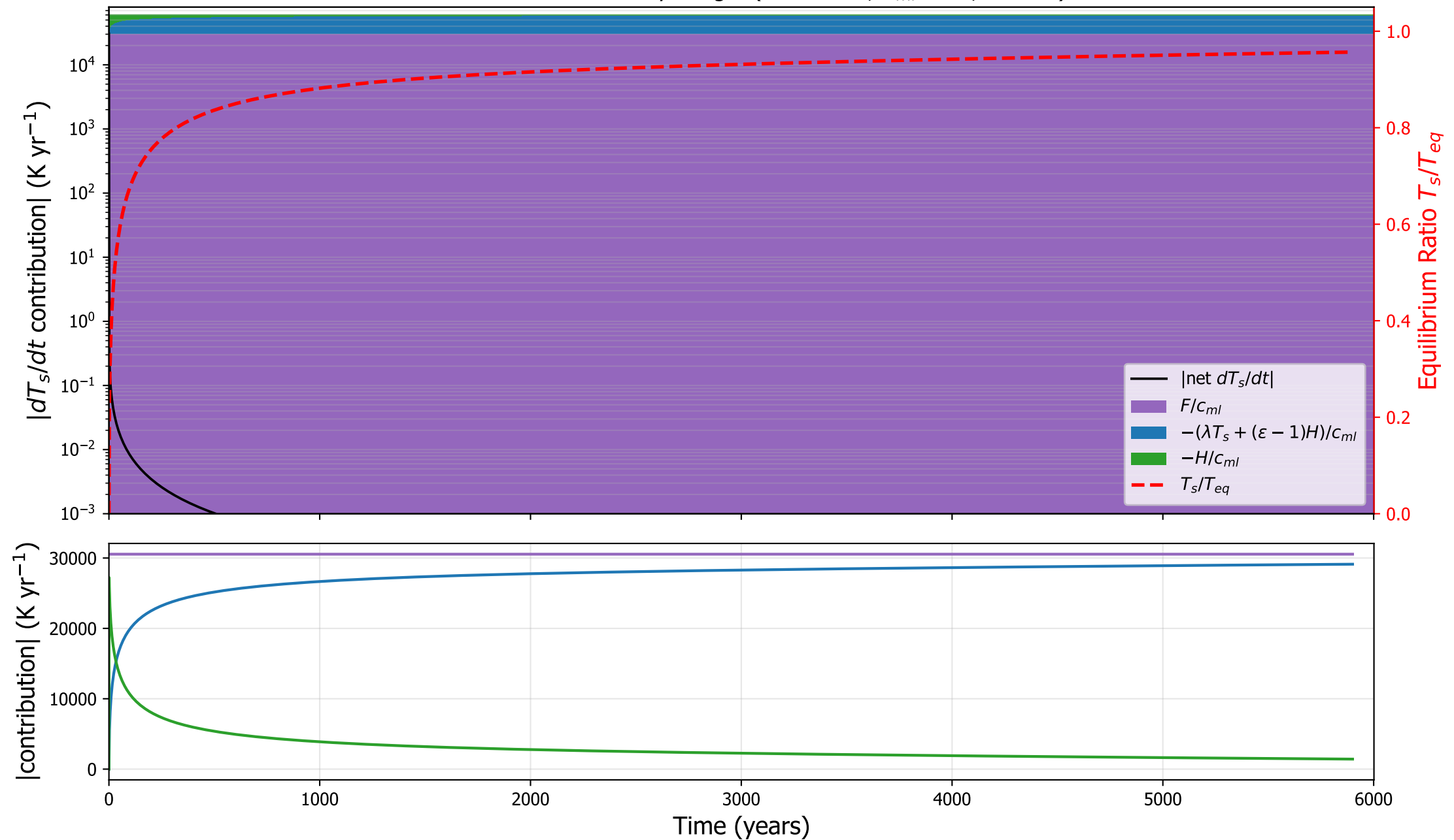
CESM1: surface tendency budget ( \kappa=3.4\text{e-}05 , h_{ml}=0 m, \varepsilon=0.93 )
