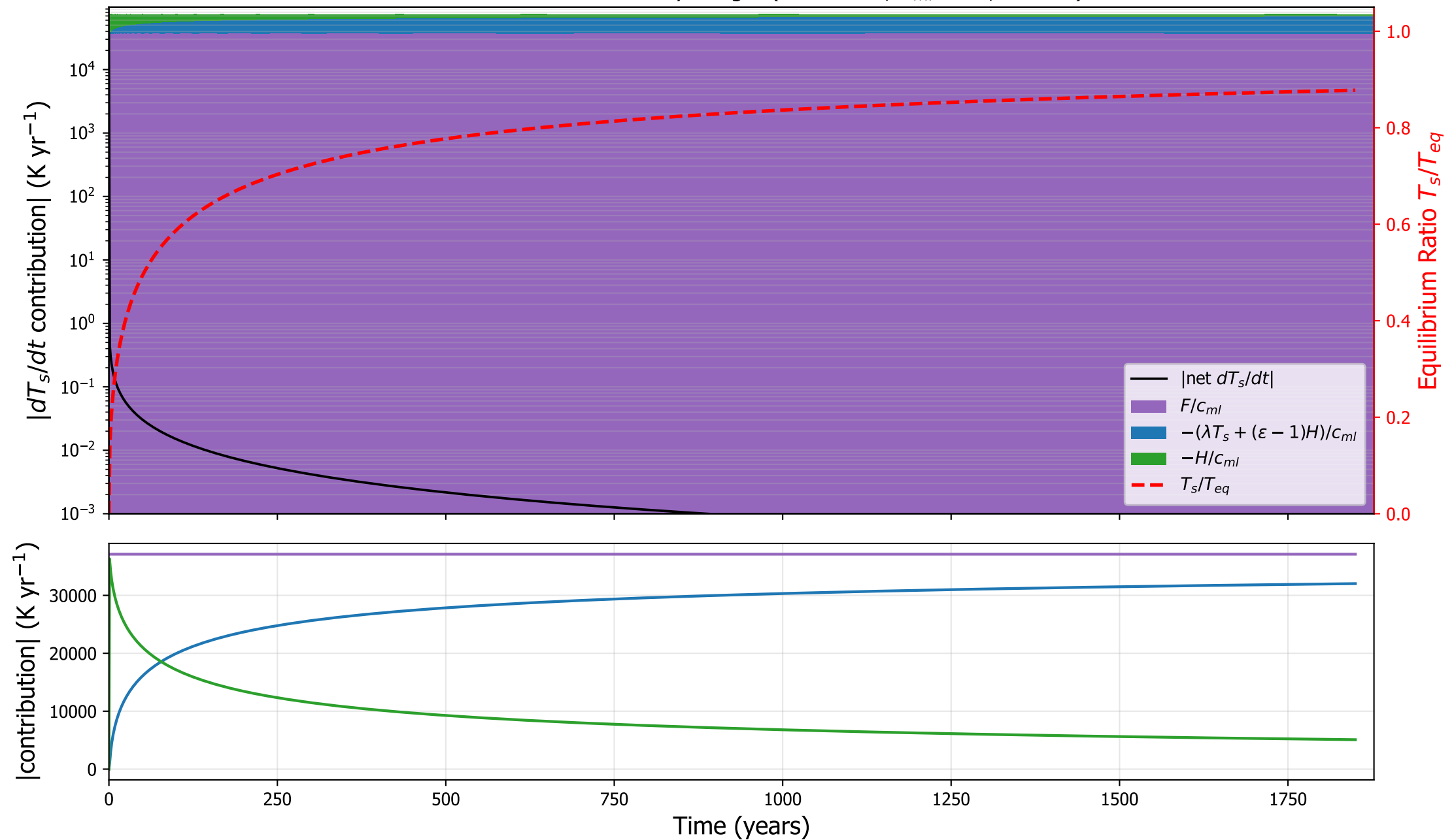
CNRMCM6: surface tendency budget ( \kappa=4.0\text{e-}05 , h_{ml}=0 m, \varepsilon=0.89 )
