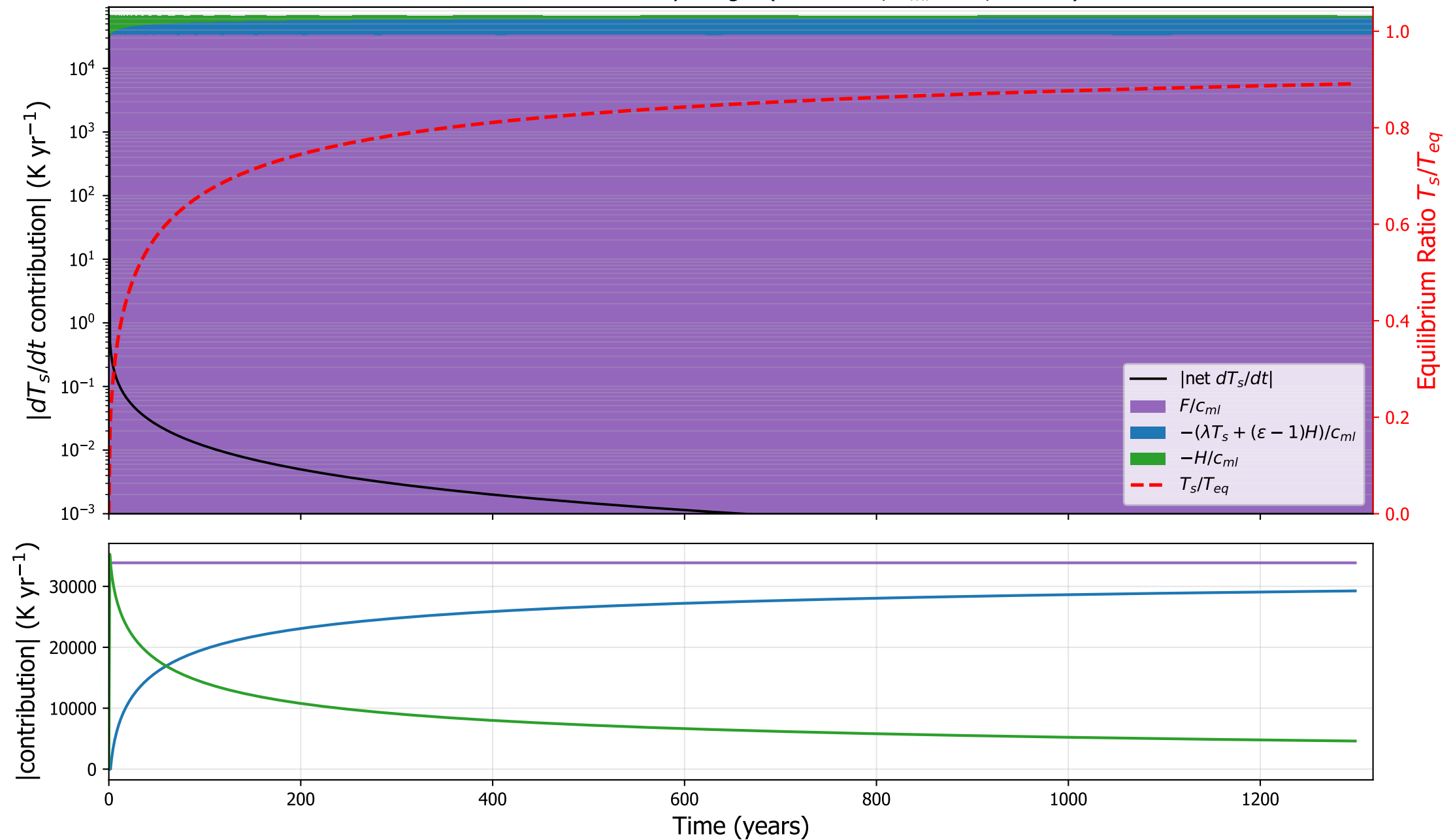
HadGEM2: surface tendency budget ( \kappa=3.3\text{e-}05 , h_{ml}=0 m, \varepsilon=0.80 )
