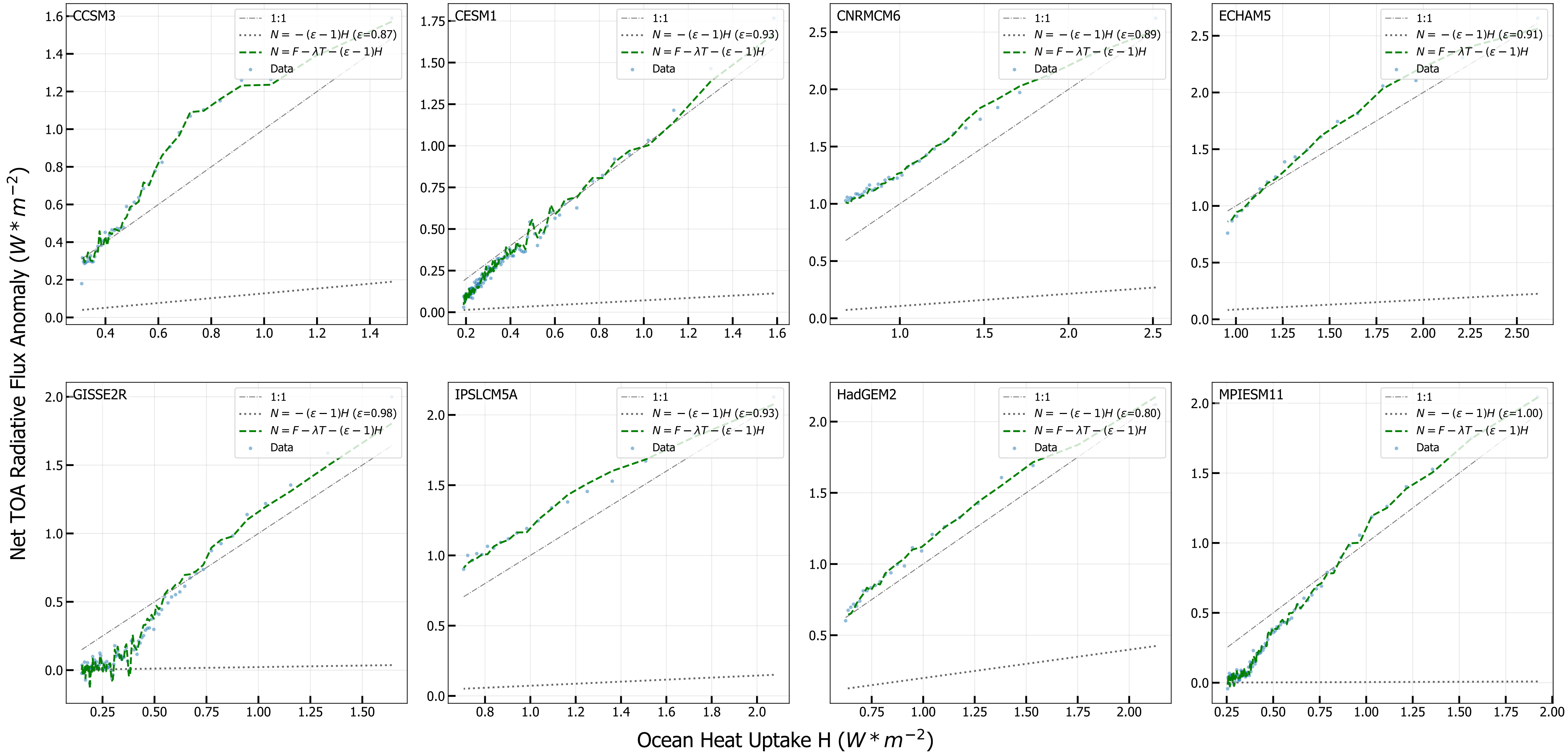
4xCO 2 Net TOA vs Ocean Heat Uptake H
