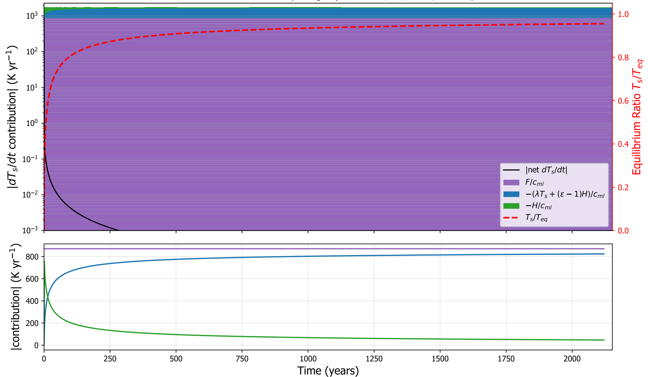
CCSM3: surface tendency budget ( \kappa=4.1\text{e-}05 , h_{ml}=0 m, \varepsilon=0.83 )
