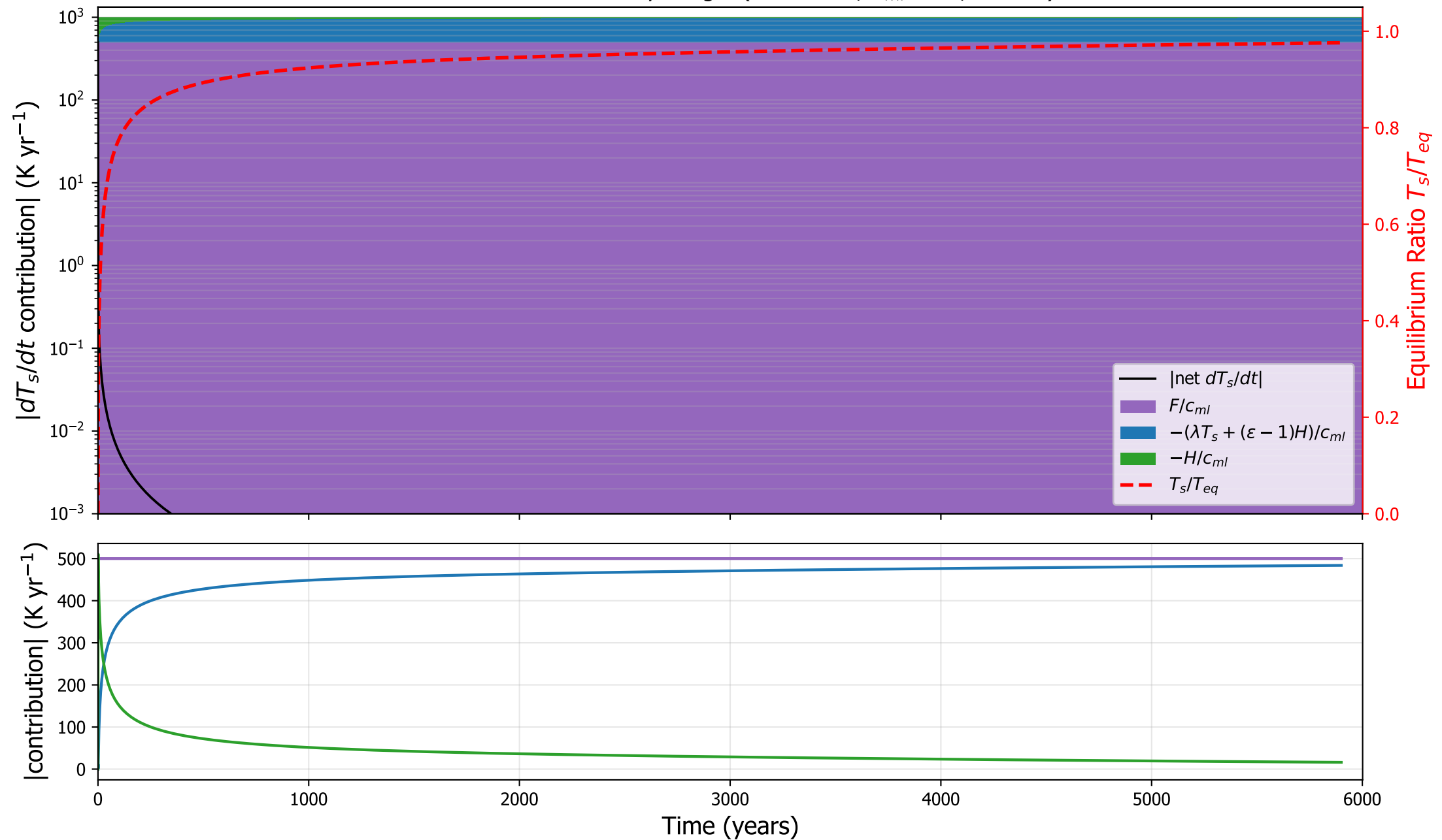
CESM1: surface tendency budget ( \kappa=4.4\text{e-}05 , h_{ml}=0 m, \varepsilon=0.74 )
