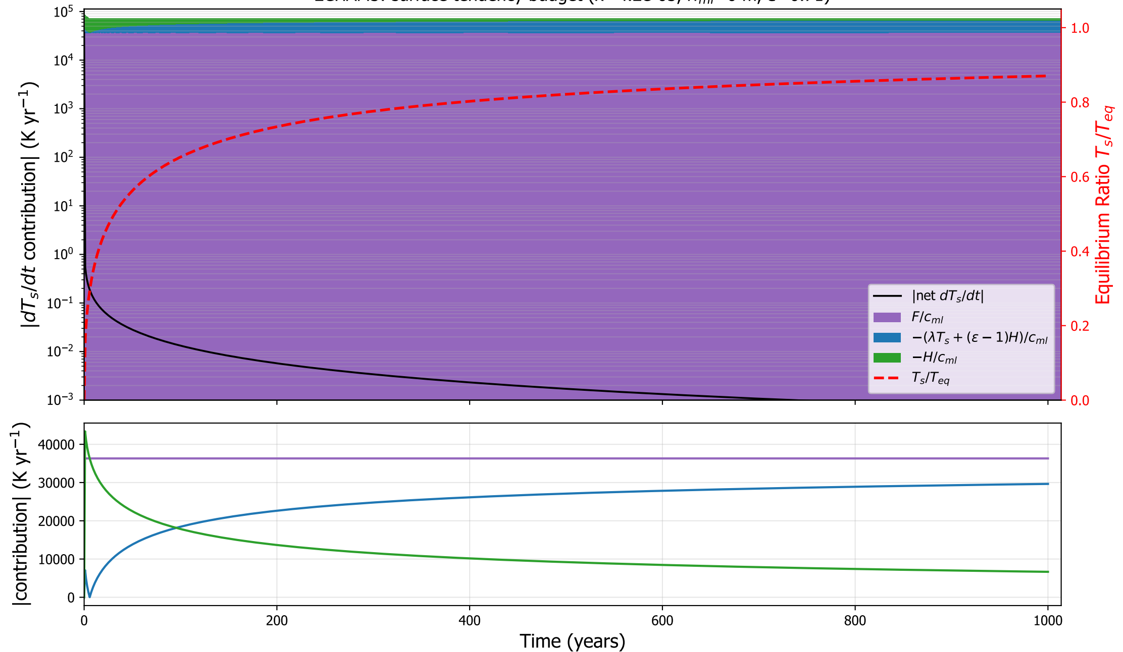
ECHAM5: surface tendency budget ( \kappa=4.2\text{e-}05 , h_{ml}=0 m, \varepsilon=0.71 )
