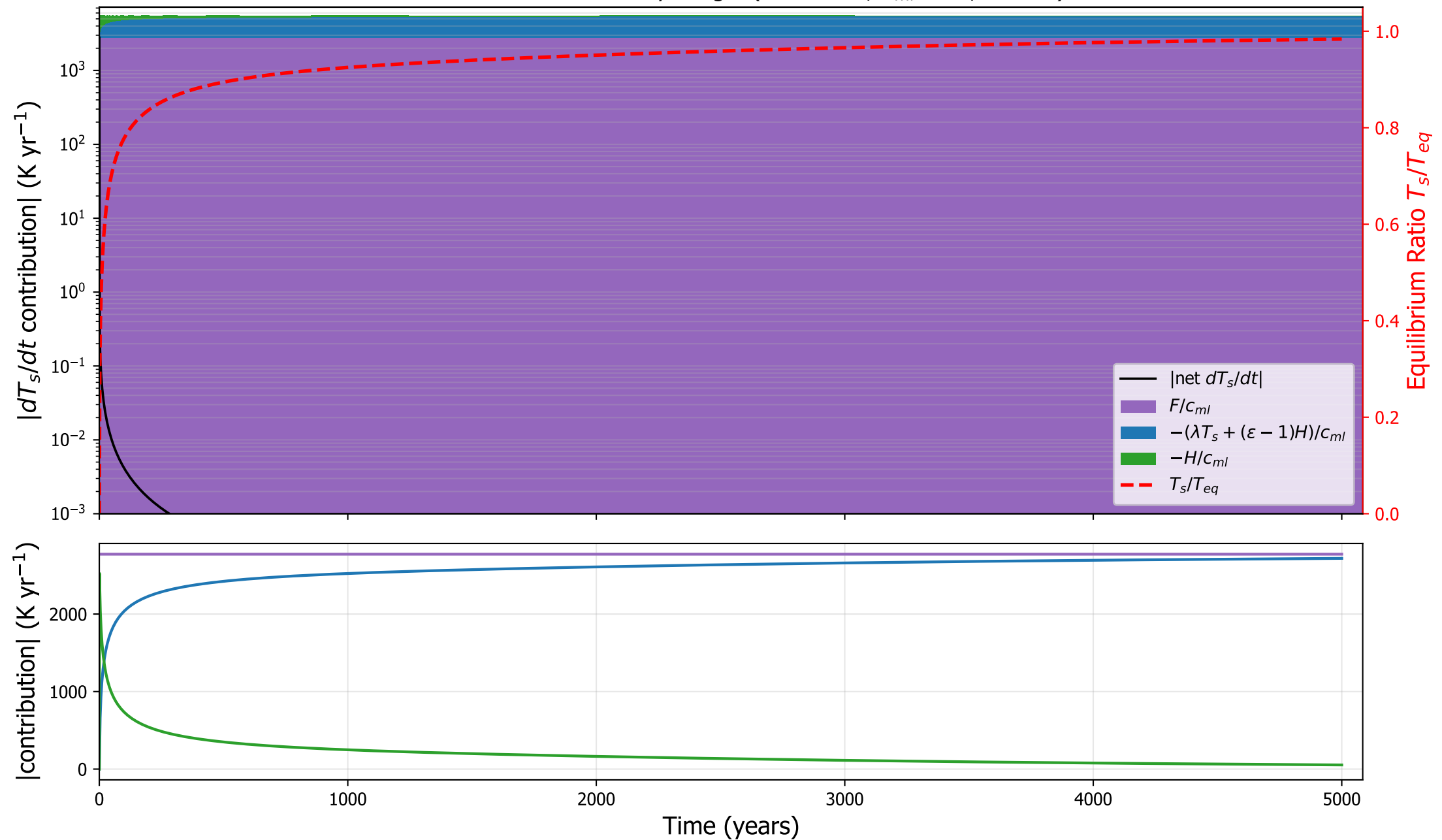
GISSE2R: surface tendency budget ( \kappa=8.5\text{e-}05 , h_{ml}=0 m, \varepsilon=0.84 )
