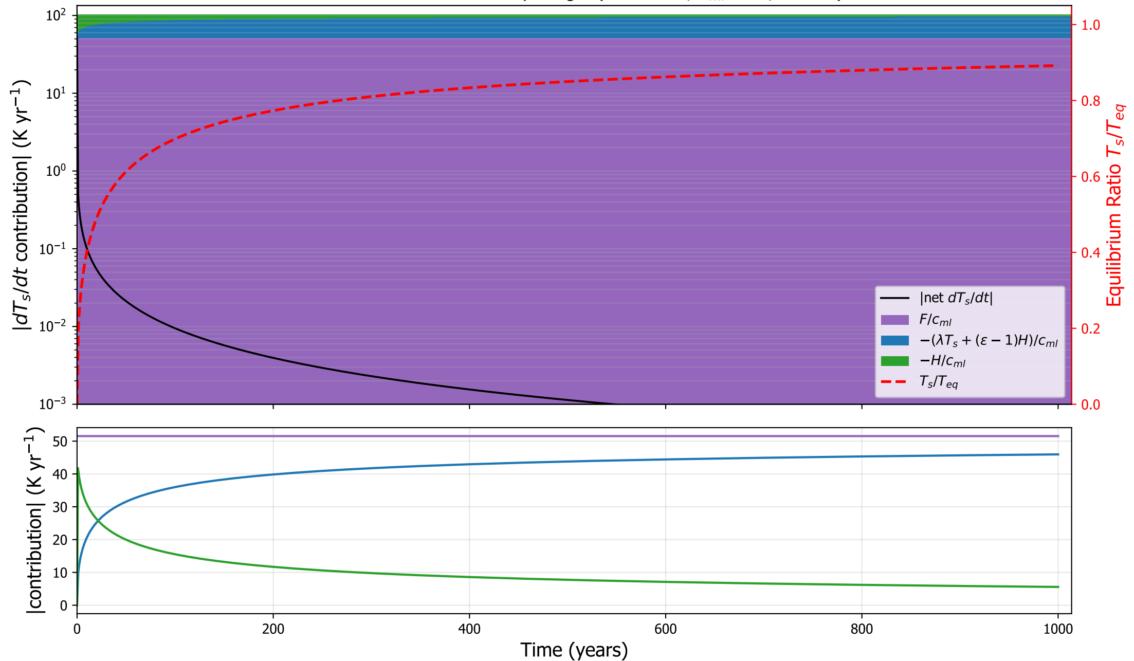
IPSLCM5A: surface tendency budget ( \kappa=4.2\text{e-}05 , h_{ml}=1 m, \varepsilon=1.00 )
