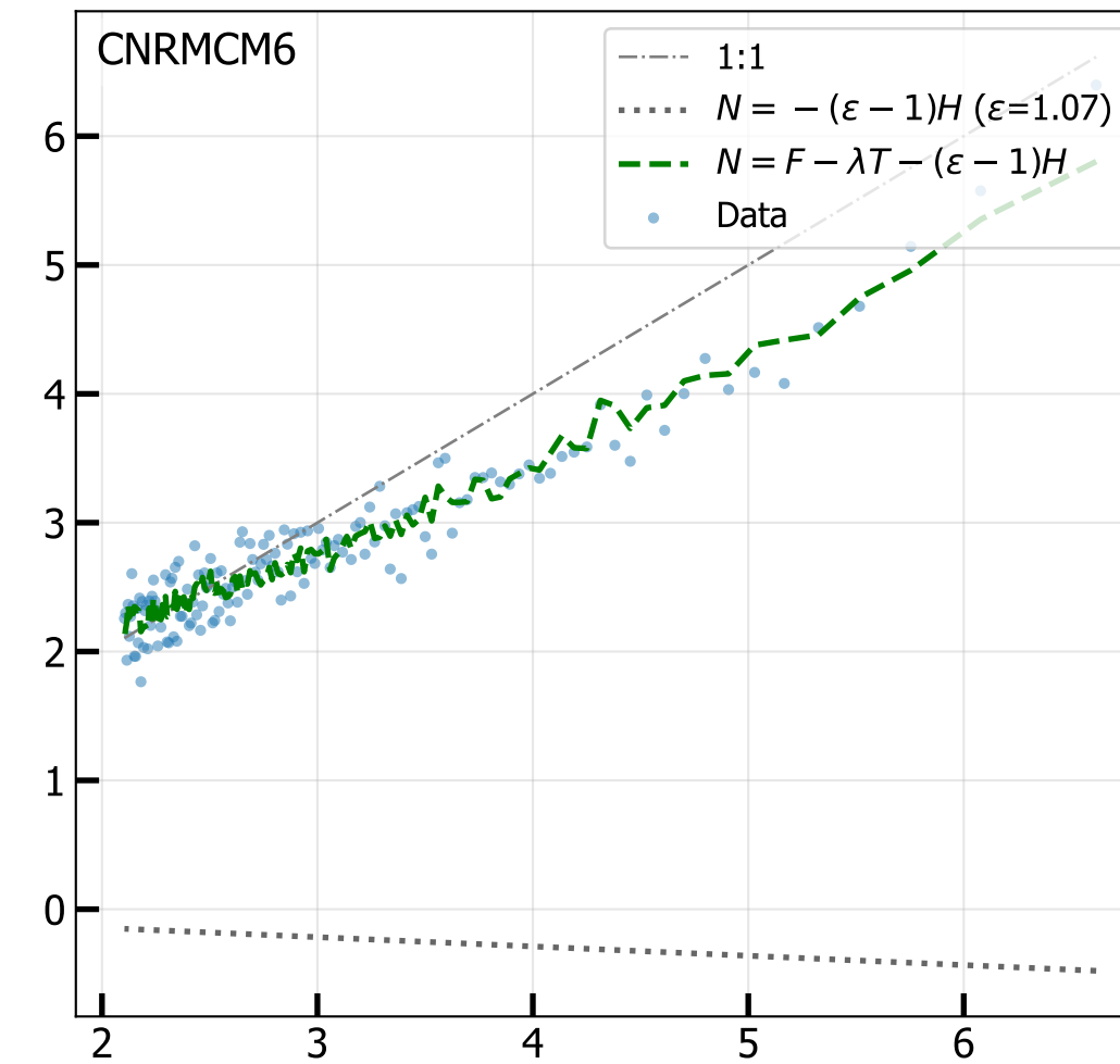
4xCO 2 Net TOA vs Ocean Heat Uptake H
