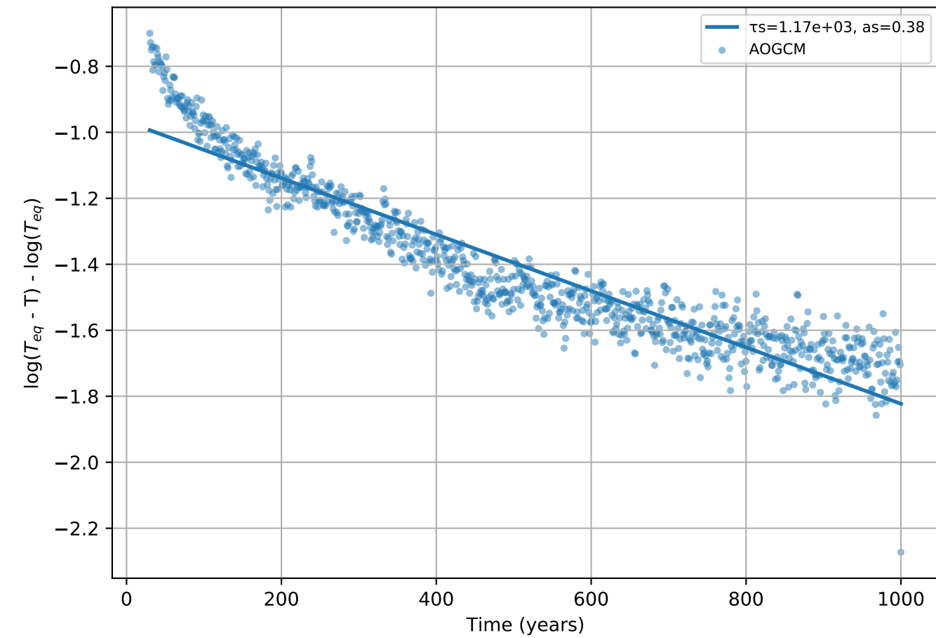
IPSLCM5A: slow mode, iter 9
