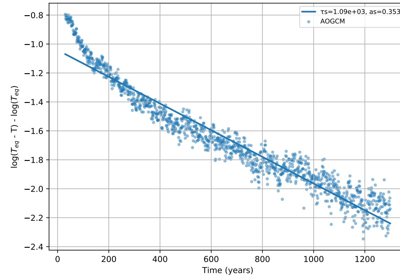
HadGEM2: slow mode, iter 9
