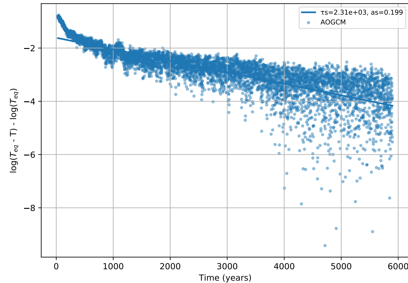
IPSLCM5A: slow mode, iter 9
