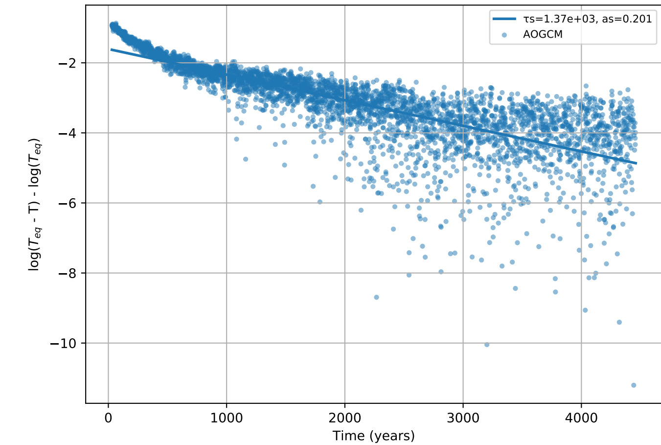
MPIESM11: slow mode, iter 9
