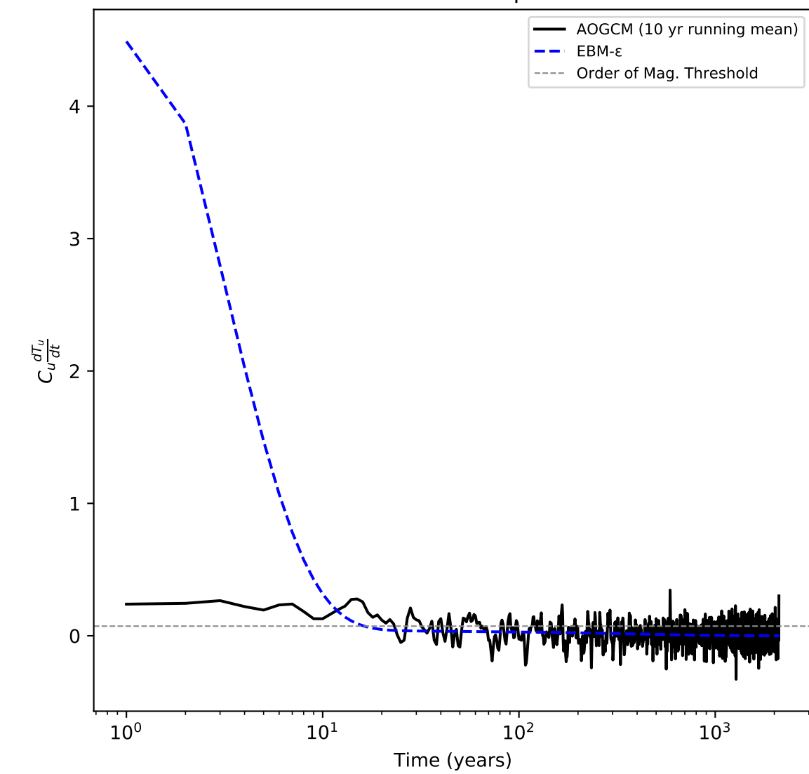
GISSER2R 4xCO2: Assumption 2 Test
