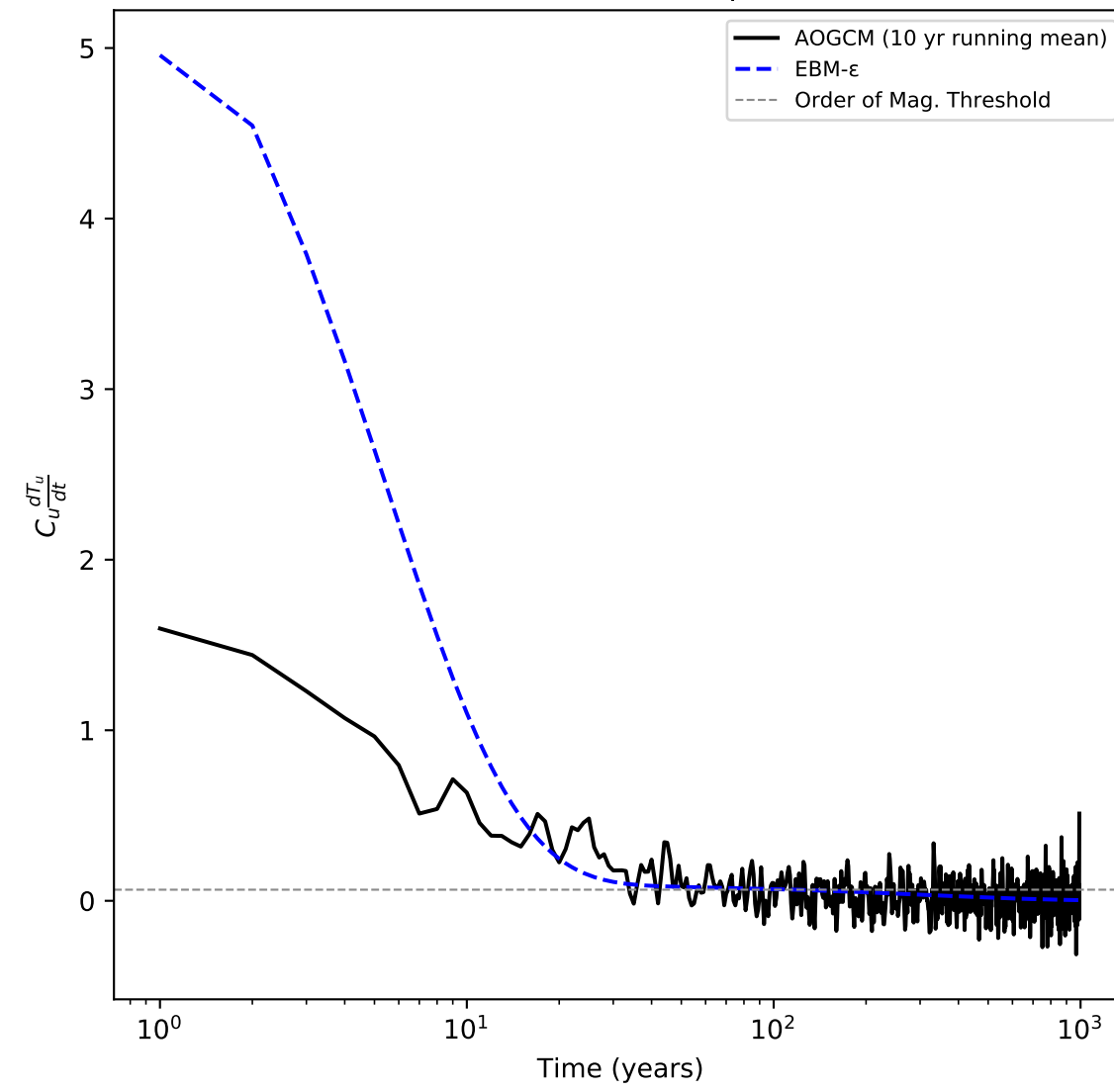
IPSLCM5A 4xCO2: Assumption 2 Test
