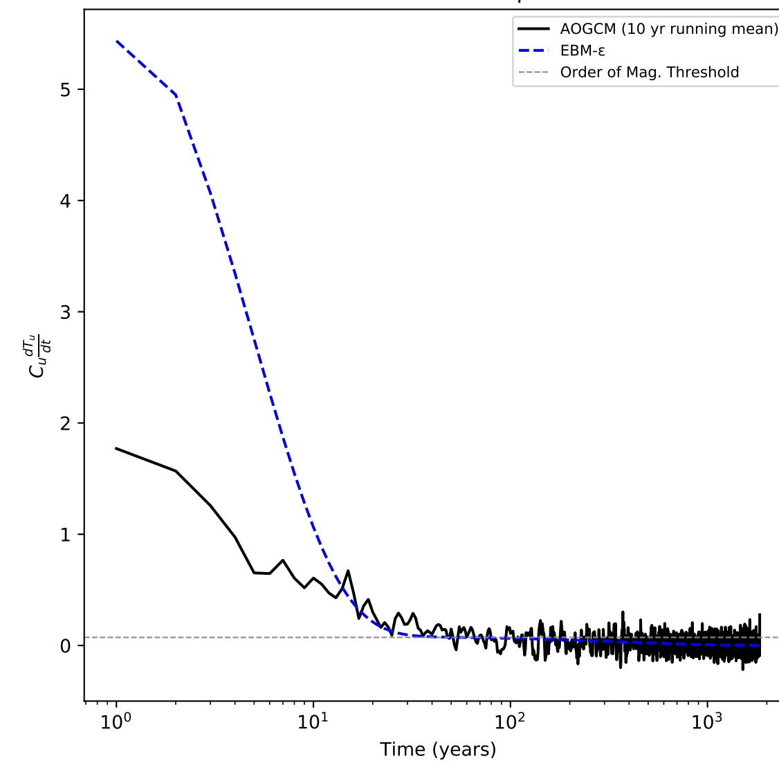
HadGEM2 4xCO2: Assumption 2 Test
