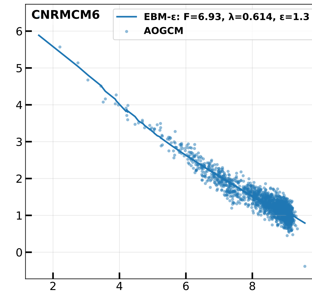
4xCO 2 Net TOA vs T 2M (radiative fit, iter 2)
