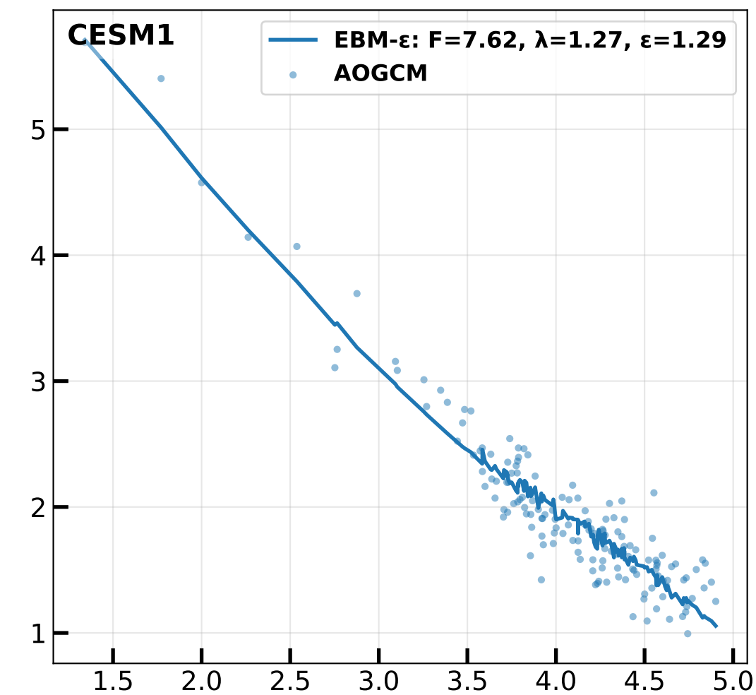
4xCO 2 Net TOA vs T 2M (radiative fit, iter 2)
