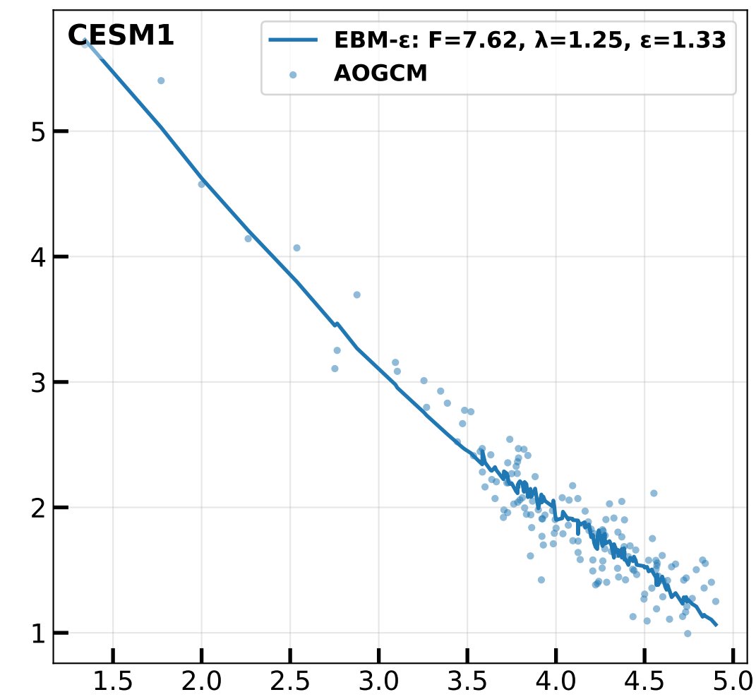
4xCO 2 Net TOA vs T 2M (radiative fit, iter 3)
