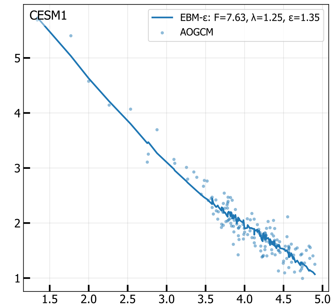
4xCO 2 Net TOA vs T 2M (radiative fit, iter 5)
