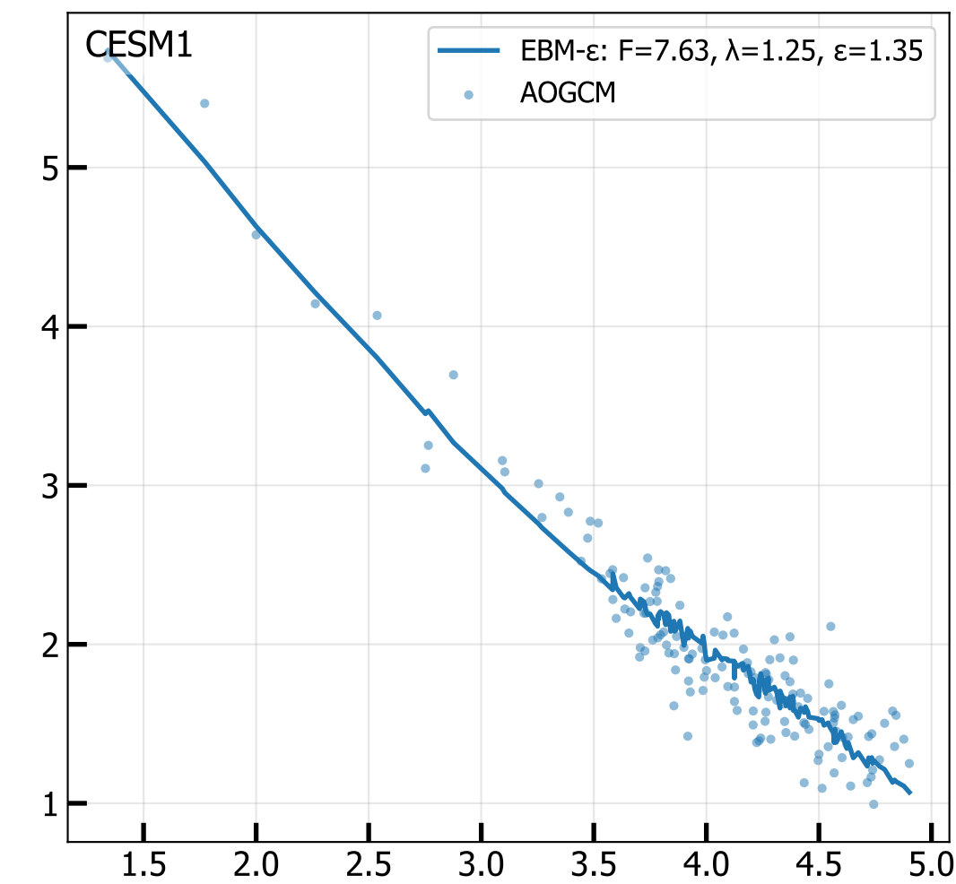
4xCO 2 Net TOA vs T 2M (radiative fit, iter 9)
