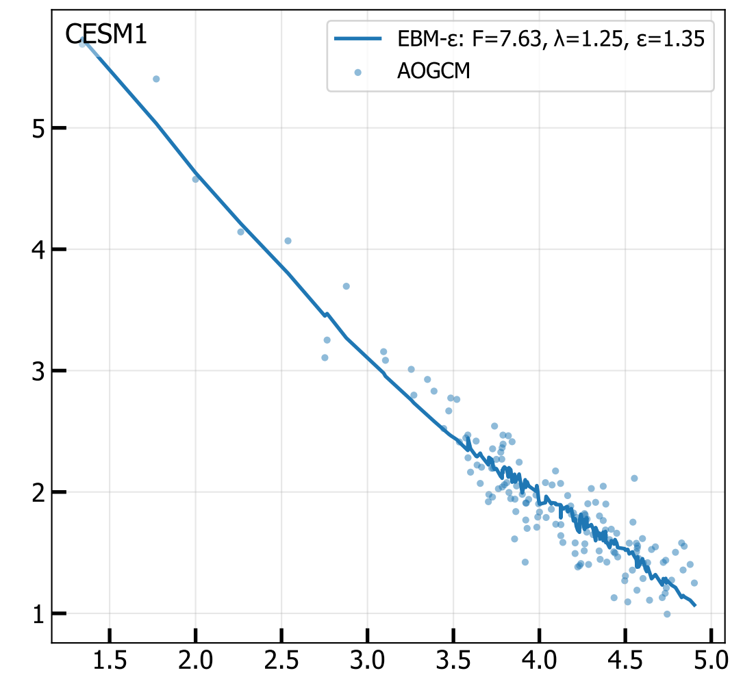
4xCO 2 Net TOA vs T 2M (radiative fit, iter 10)
