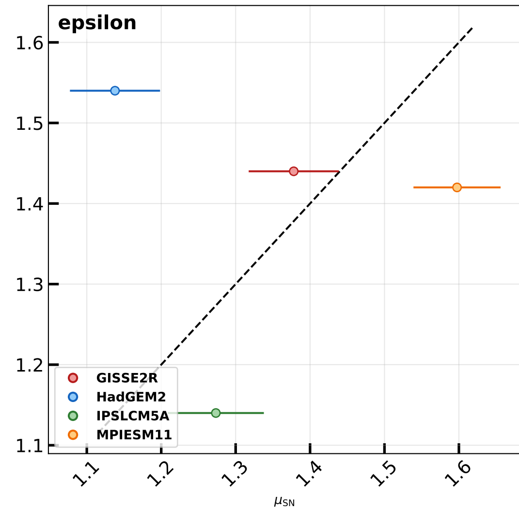
Geoffroy vs. replication (w/ 95% CI)
