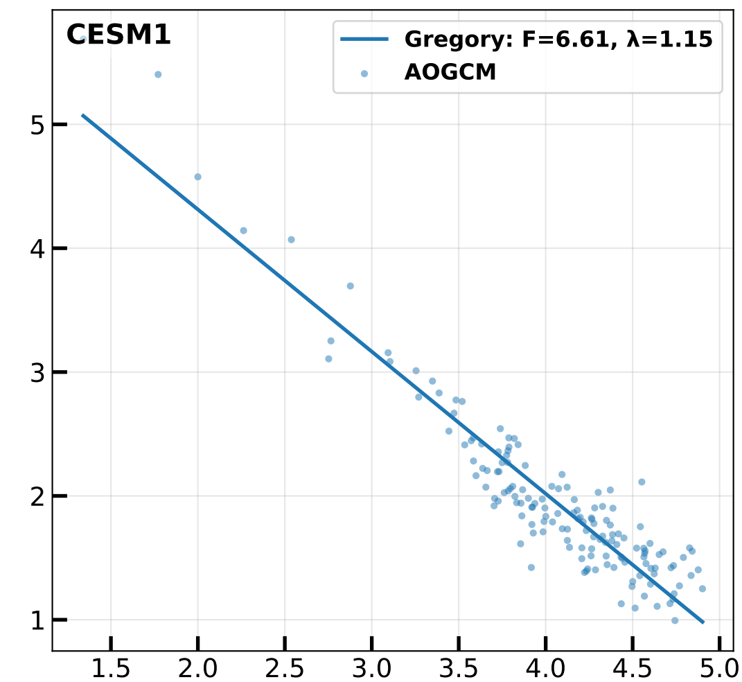
4xCO 2 Net TOA vs T 2M (radiative fit, iter 1)
