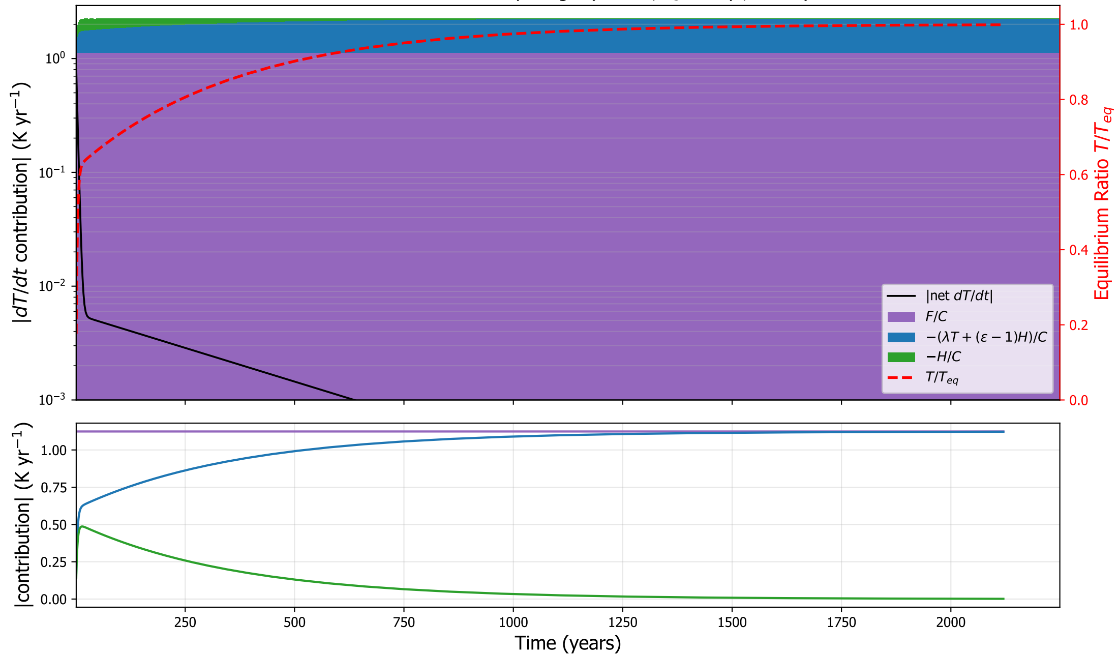
CCSM3: surface tendency budget ( \varepsilon=0.83 , \tau_s=367 yr, C=3.9 )
