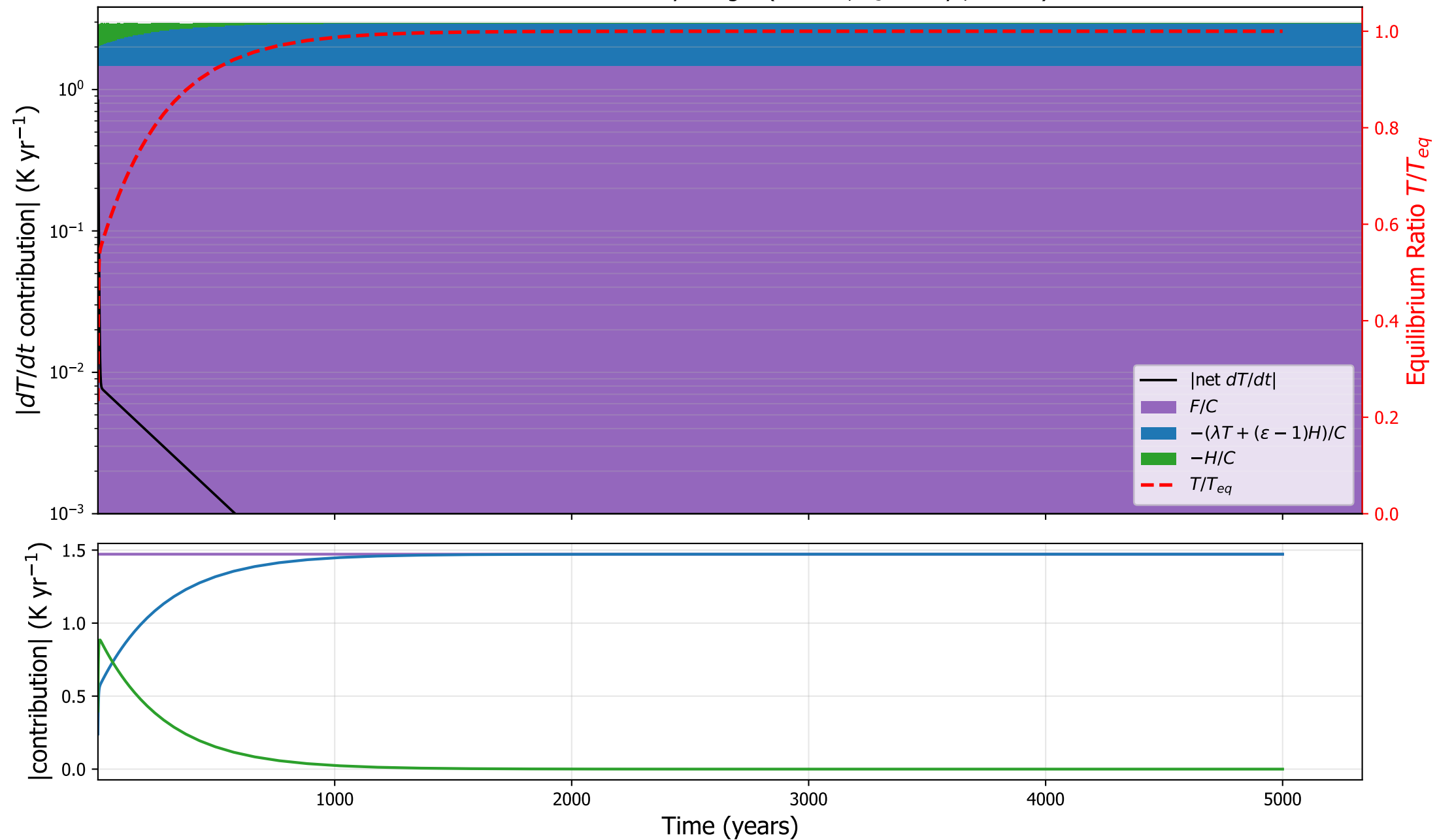
GISSE2R: surface tendency budget ( \varepsilon=0.74 , \tau_s=276 yr, C=2.8 )
