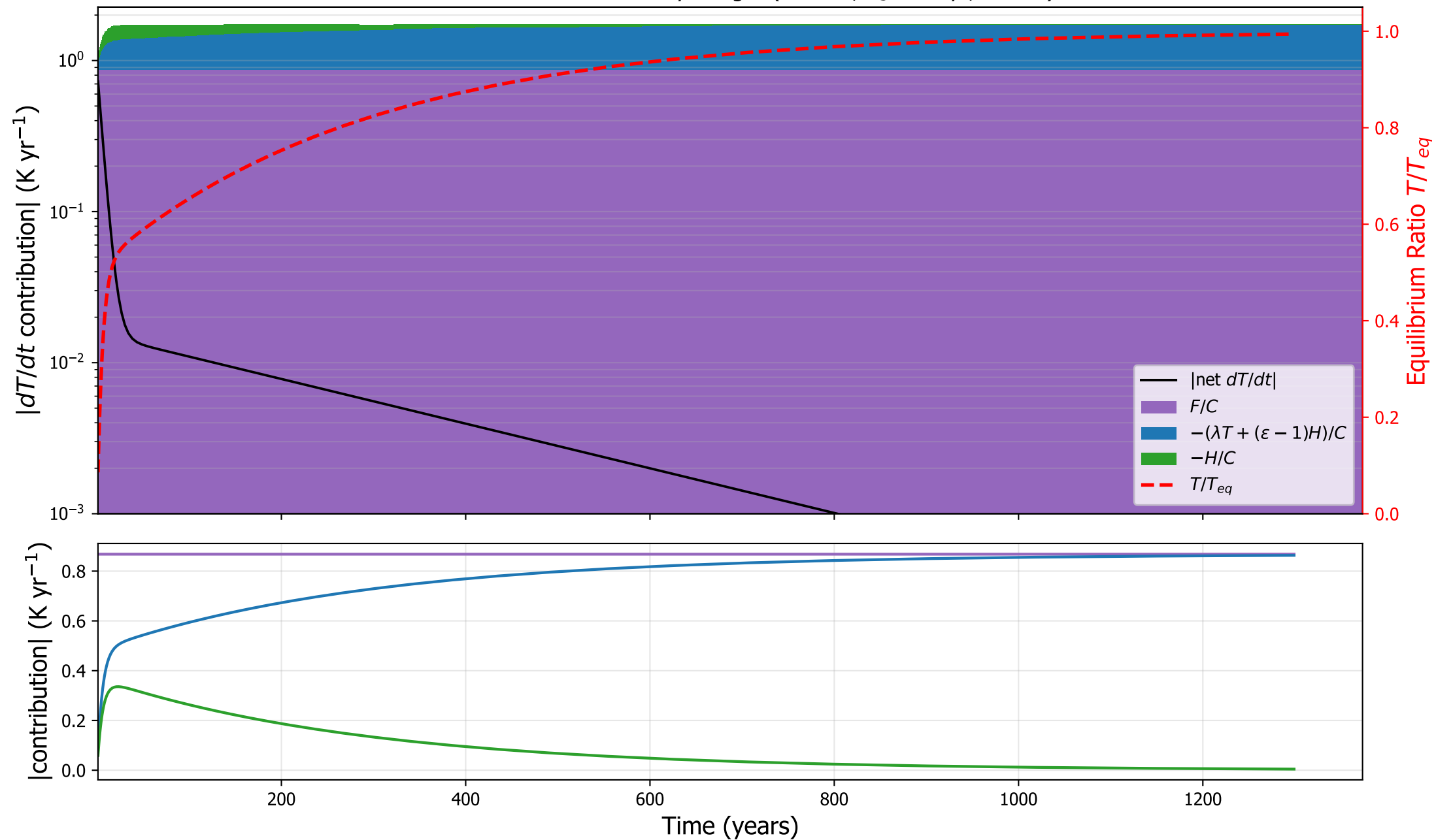
HadGEM2: surface tendency budget ( \varepsilon=1.10 , \tau_s=294 yr, C=7.1 )
