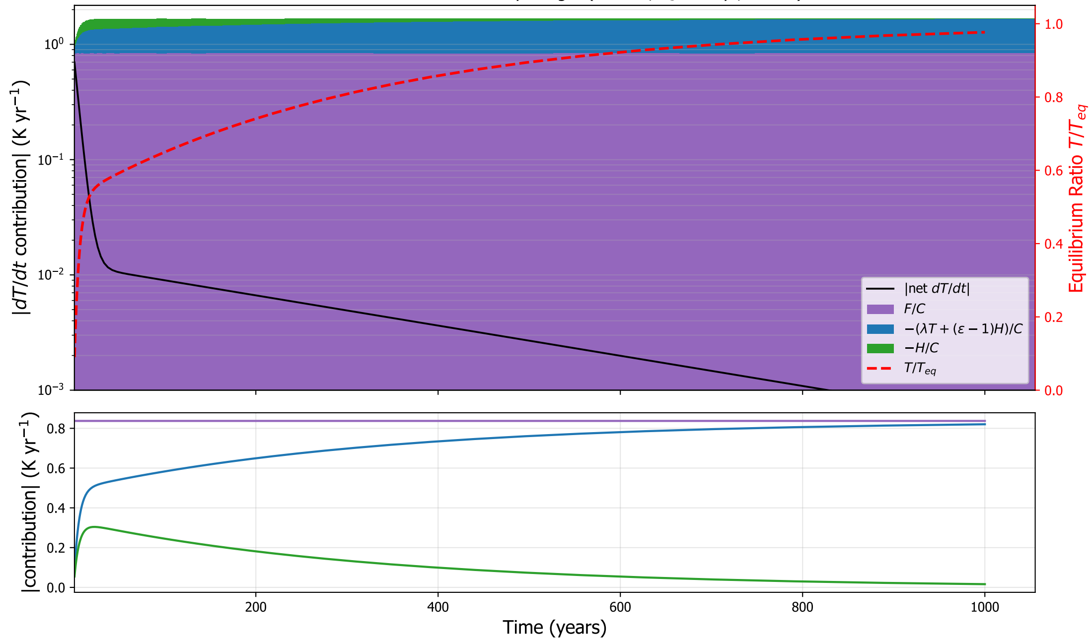
IPSLCM5A: surface tendency budget ( \varepsilon=1.16 , \tau_s=332 yr, C=7.8 )
