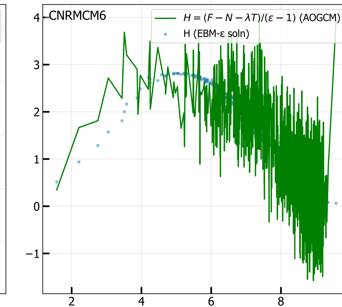
4xCO 2 Ocean Heat Uptake H vs T 2M (radiative fit, iter 2)
