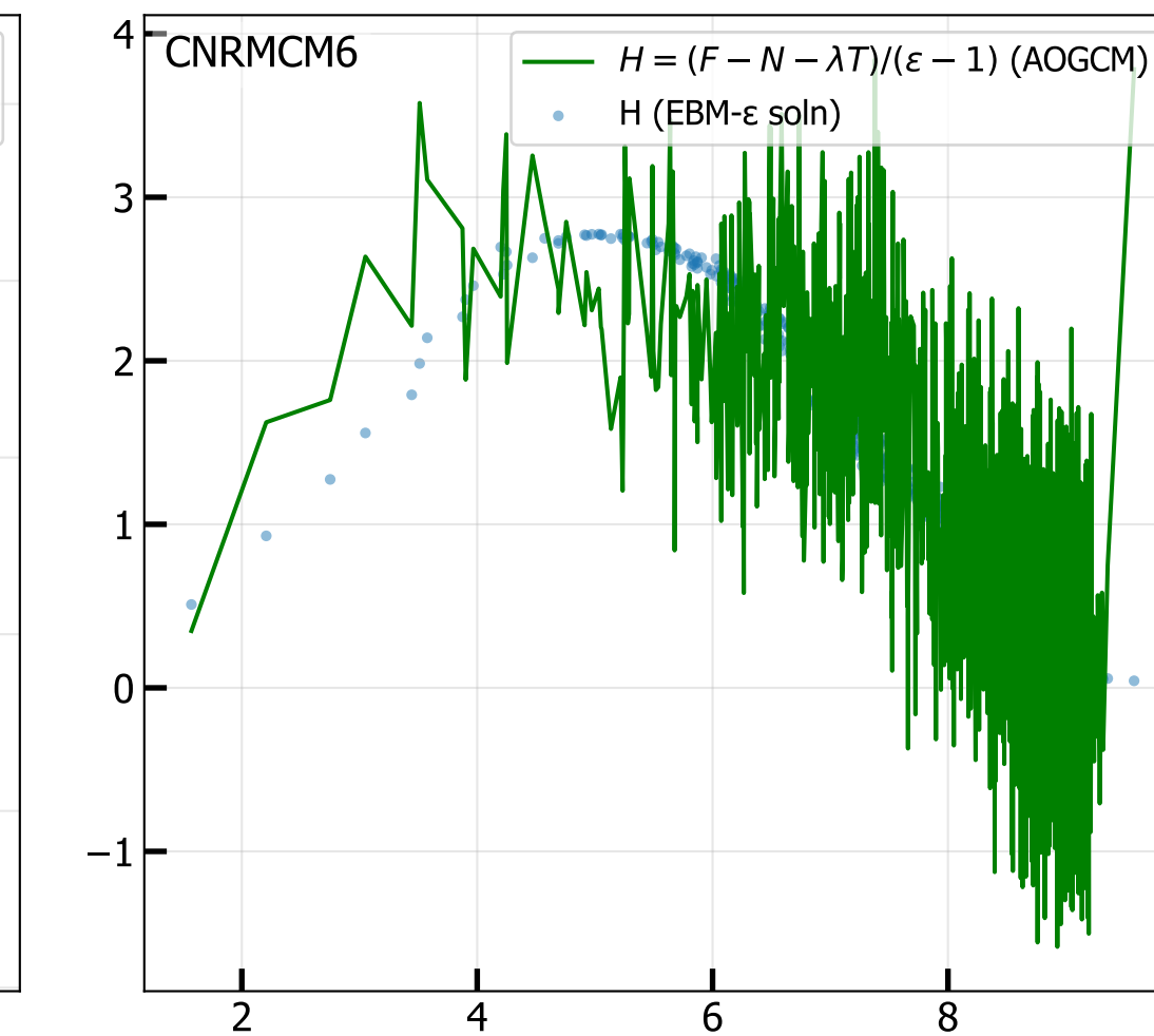
4xCO 2 Ocean Heat Uptake H vs T 2M (radiative fit, iter 3)
