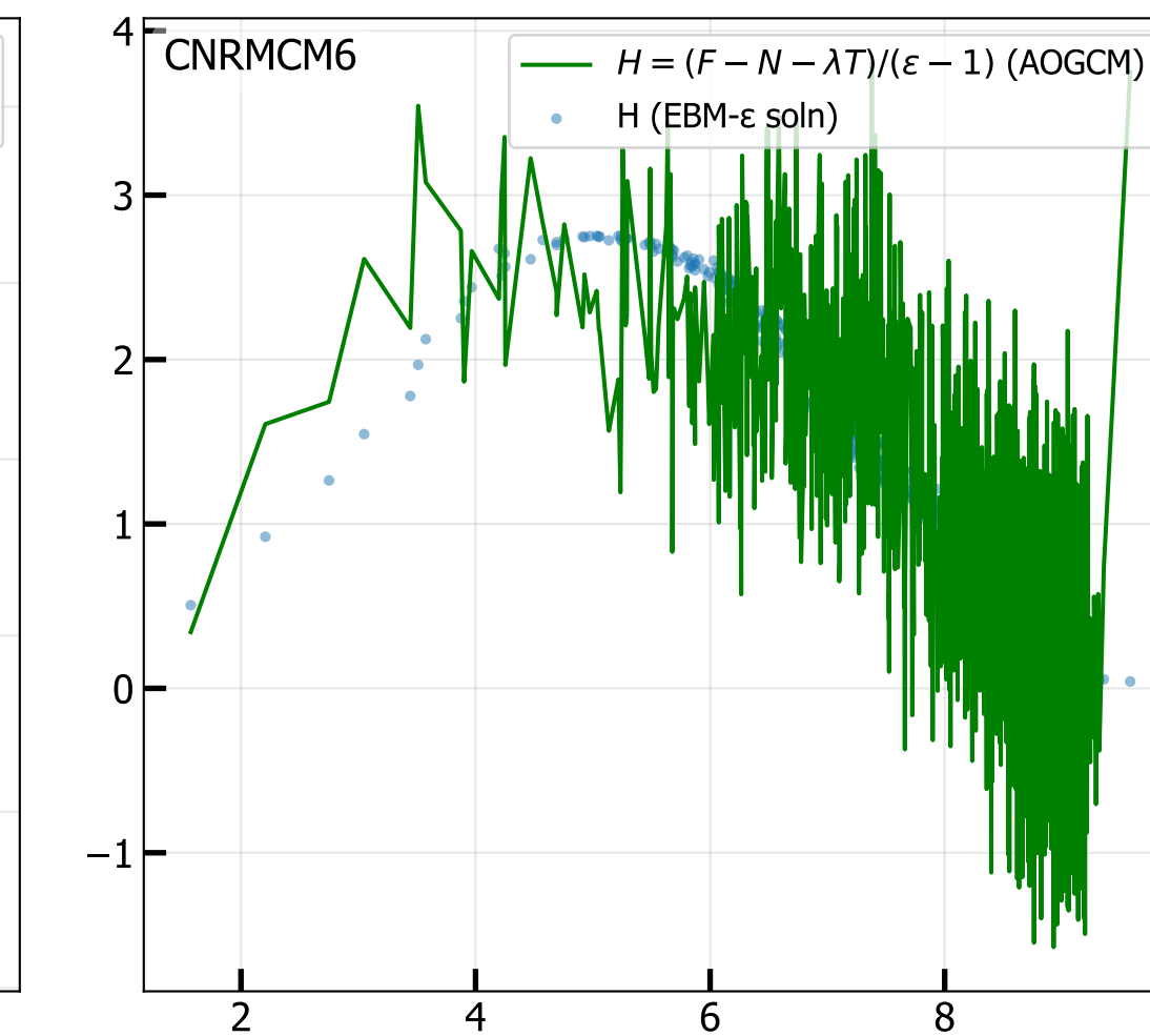
4xCO 2 Ocean Heat Uptake H vs T 2M (radiative fit, iter 4)
