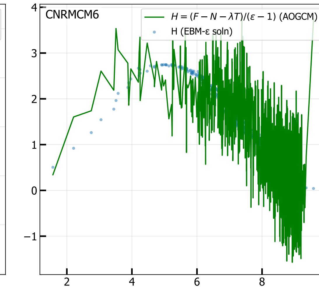
4xCO 2 Ocean Heat Uptake H vs T 2M (radiative fit, iter 5)
