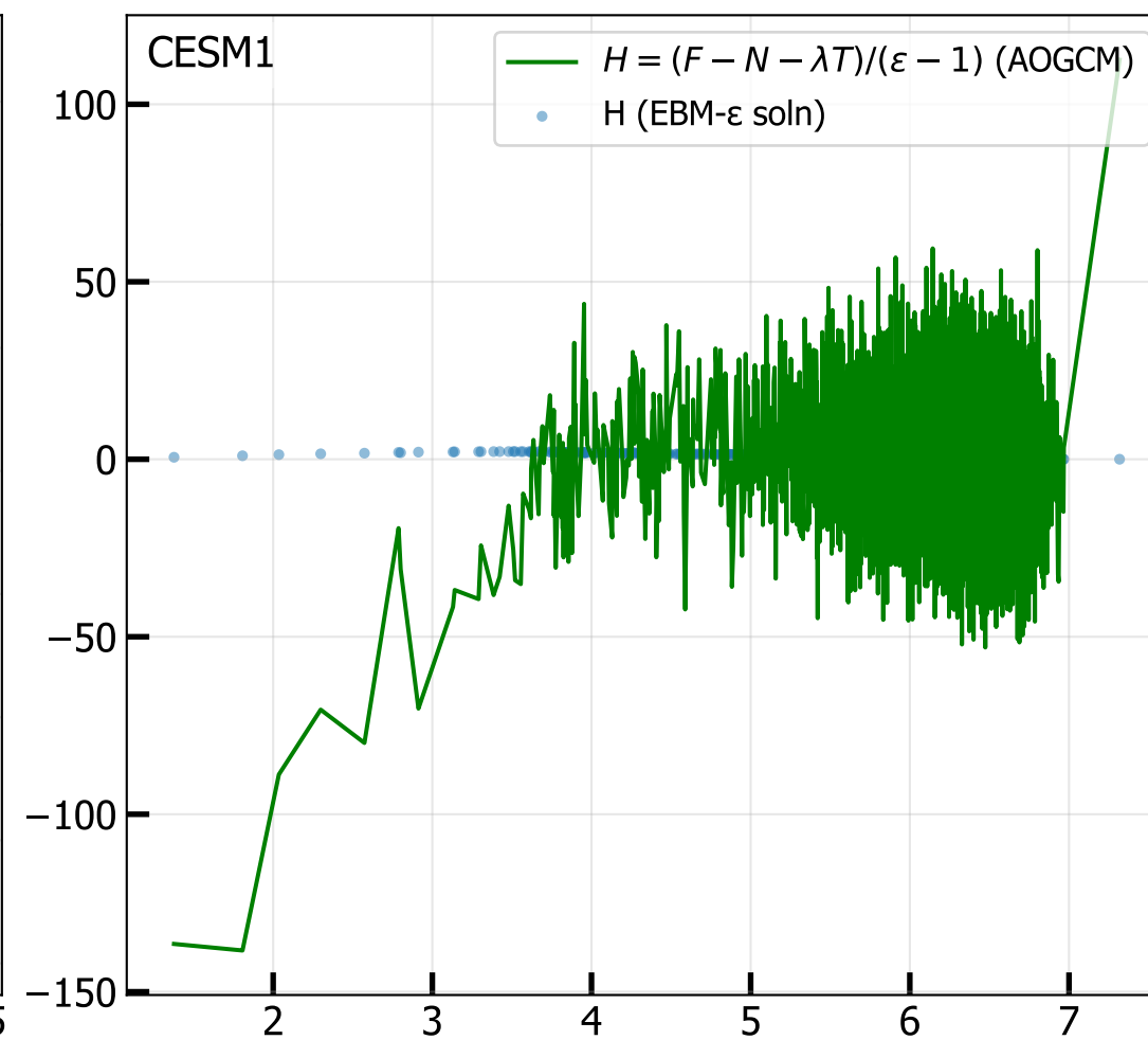
4xCO 2 Ocean Heat Uptake H vs T 2M (radiative fit, iter 6)
