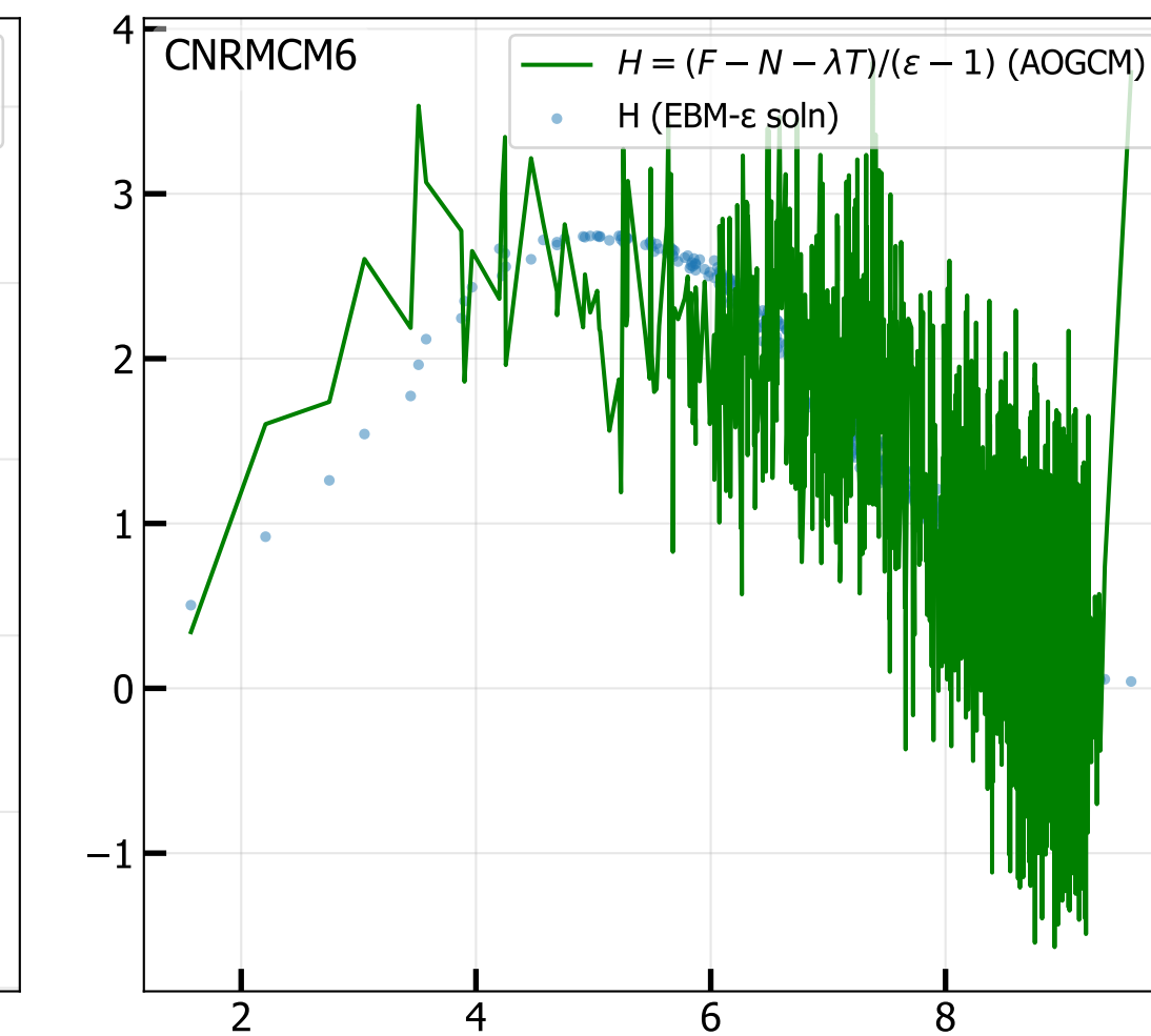
4xCO 2 Ocean Heat Uptake H vs T 2M (radiative fit, iter 7)
