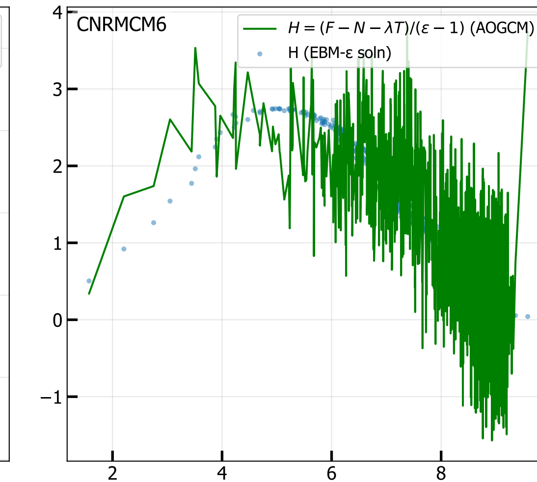
4xCO 2 Ocean Heat Uptake H vs T 2M (radiative fit, iter 8)
