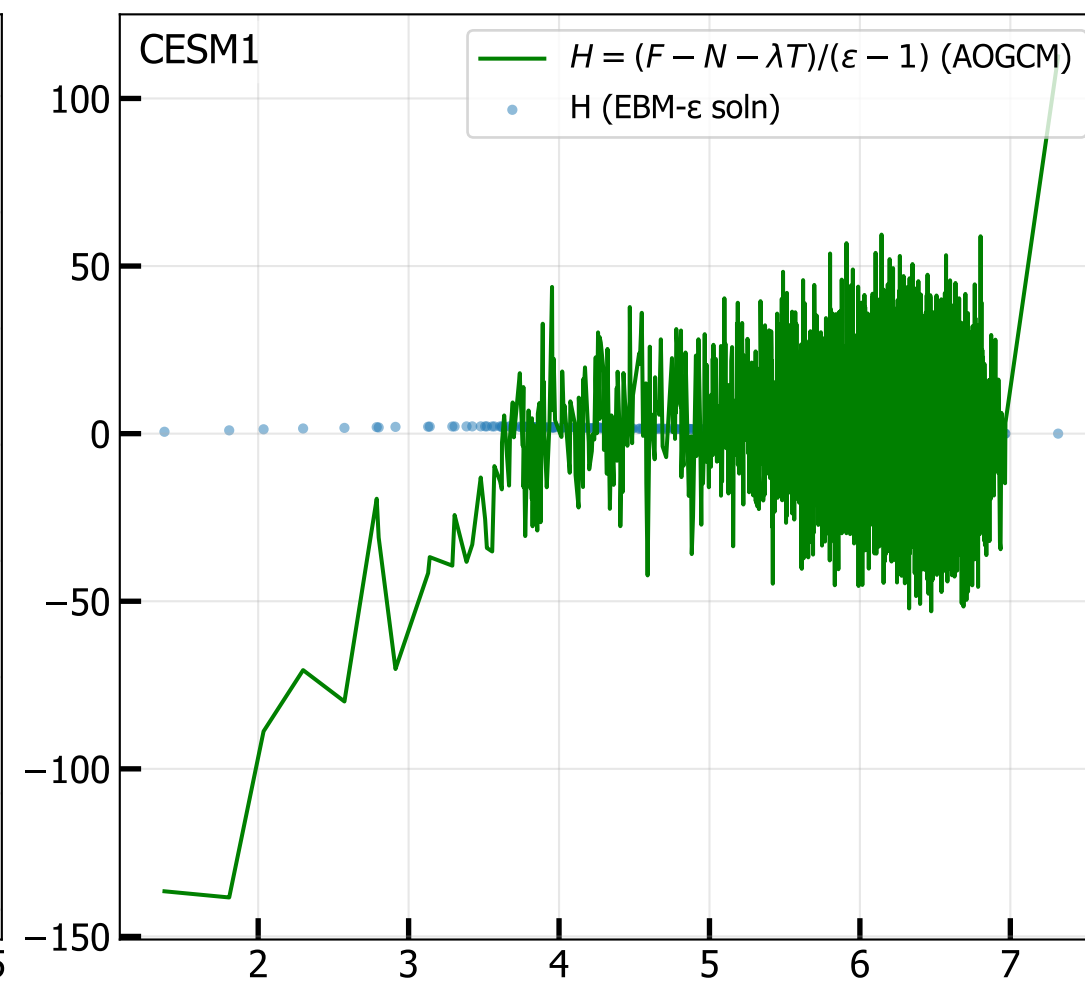
4xCO 2 Ocean Heat Uptake H vs T 2M (radiative fit, iter 9)
