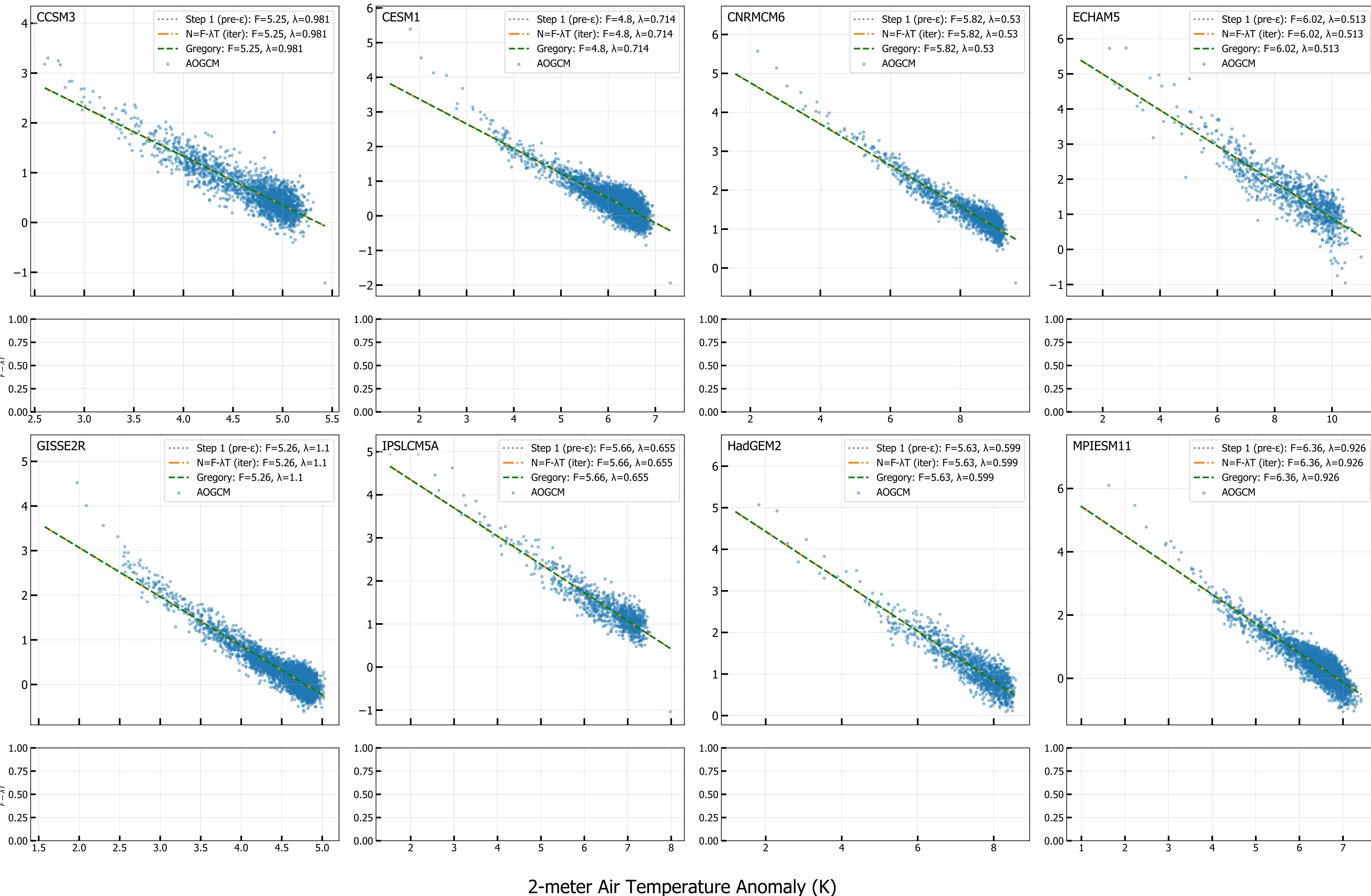
4xCO 2 Net TOA vs T 2M (radiative fit, iter 1)
