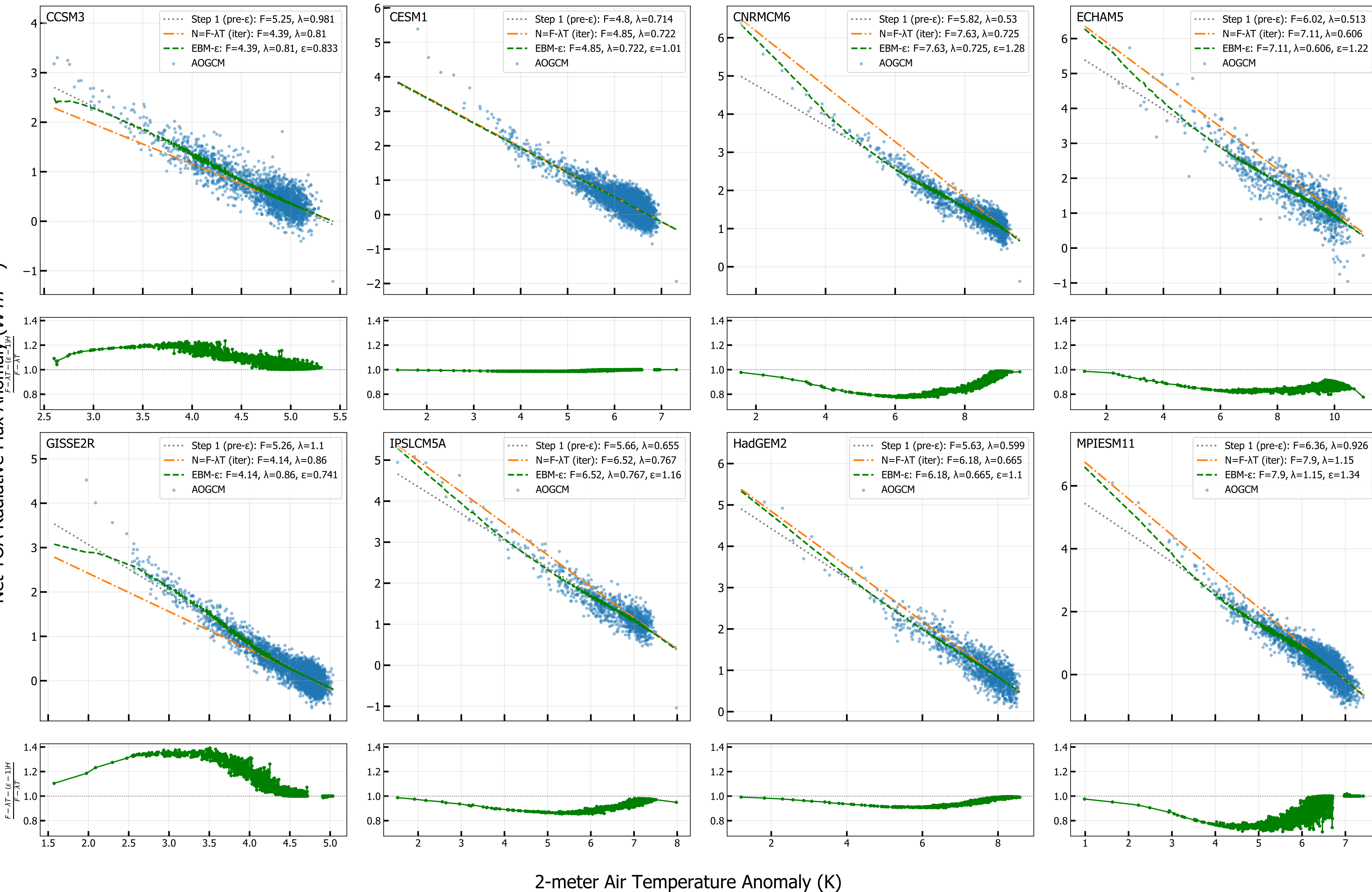
4xCO 2 Net TOA vs T 2M (radiative fit, iter 5)
