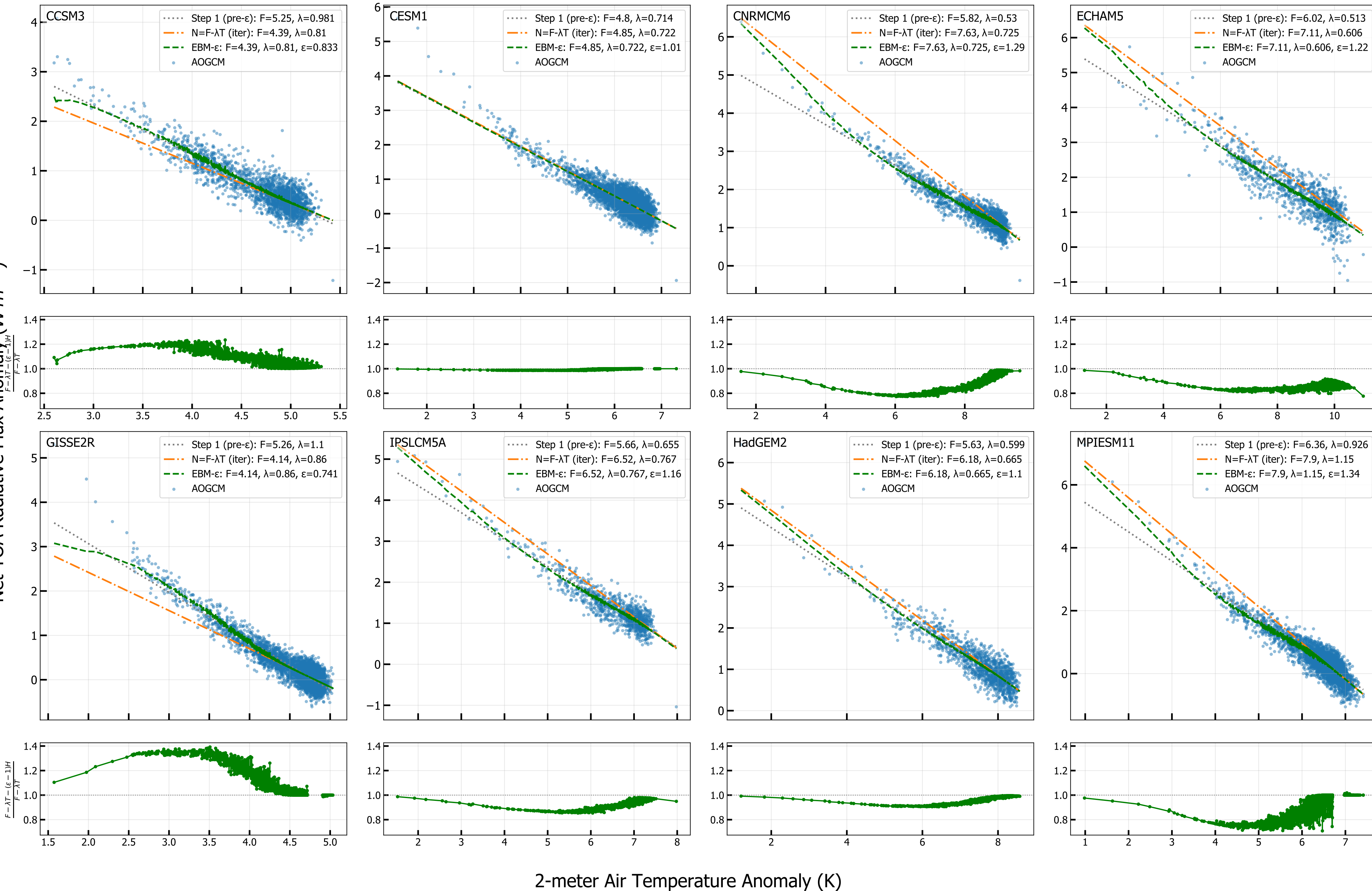
4xCO 2 Net TOA vs T 2M (radiative fit, iter 8)
