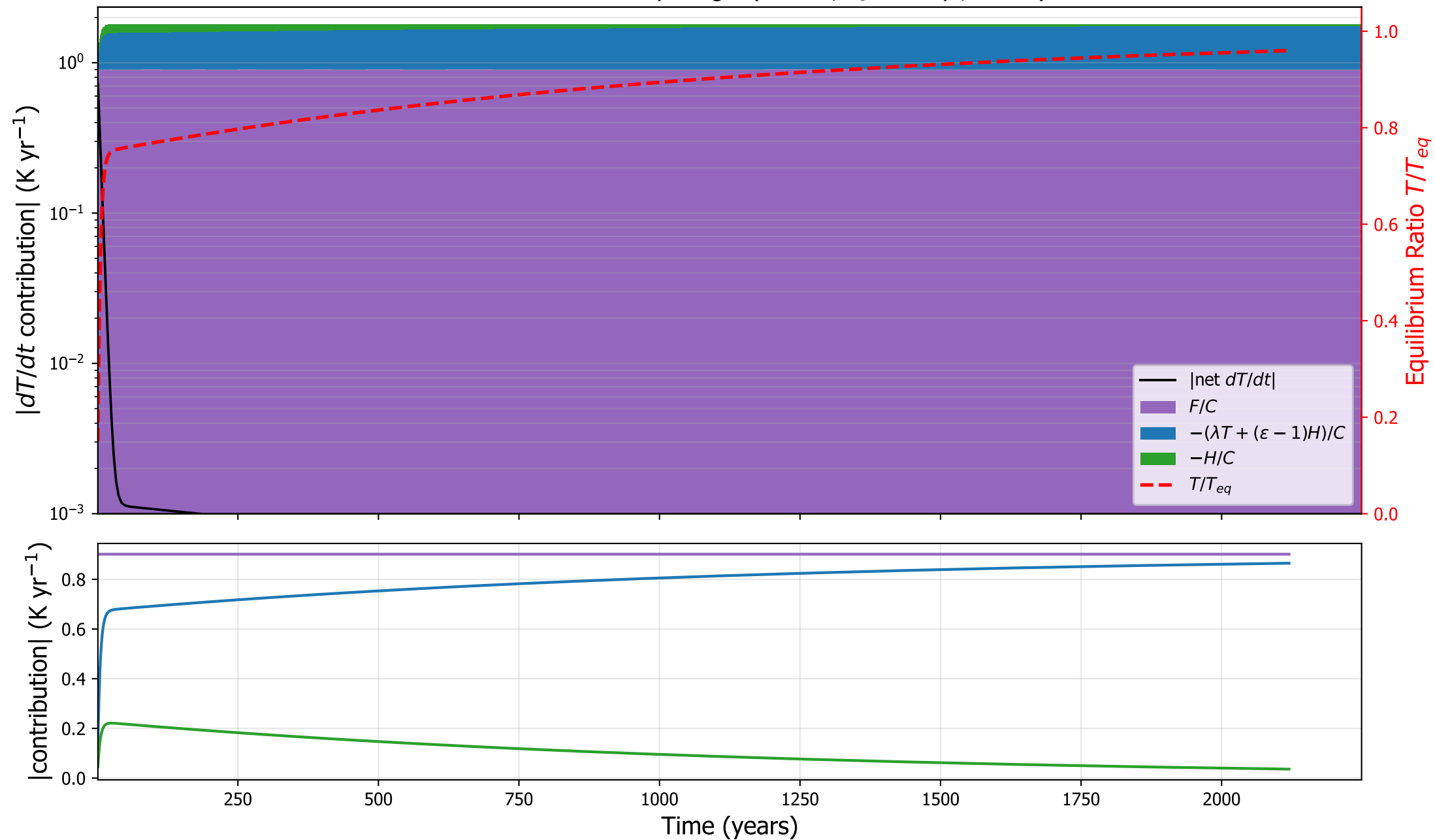
CCSM3: surface tendency budget ( \varepsilon=1.00 , \tau_s=1153 yr, C=5.8 )
