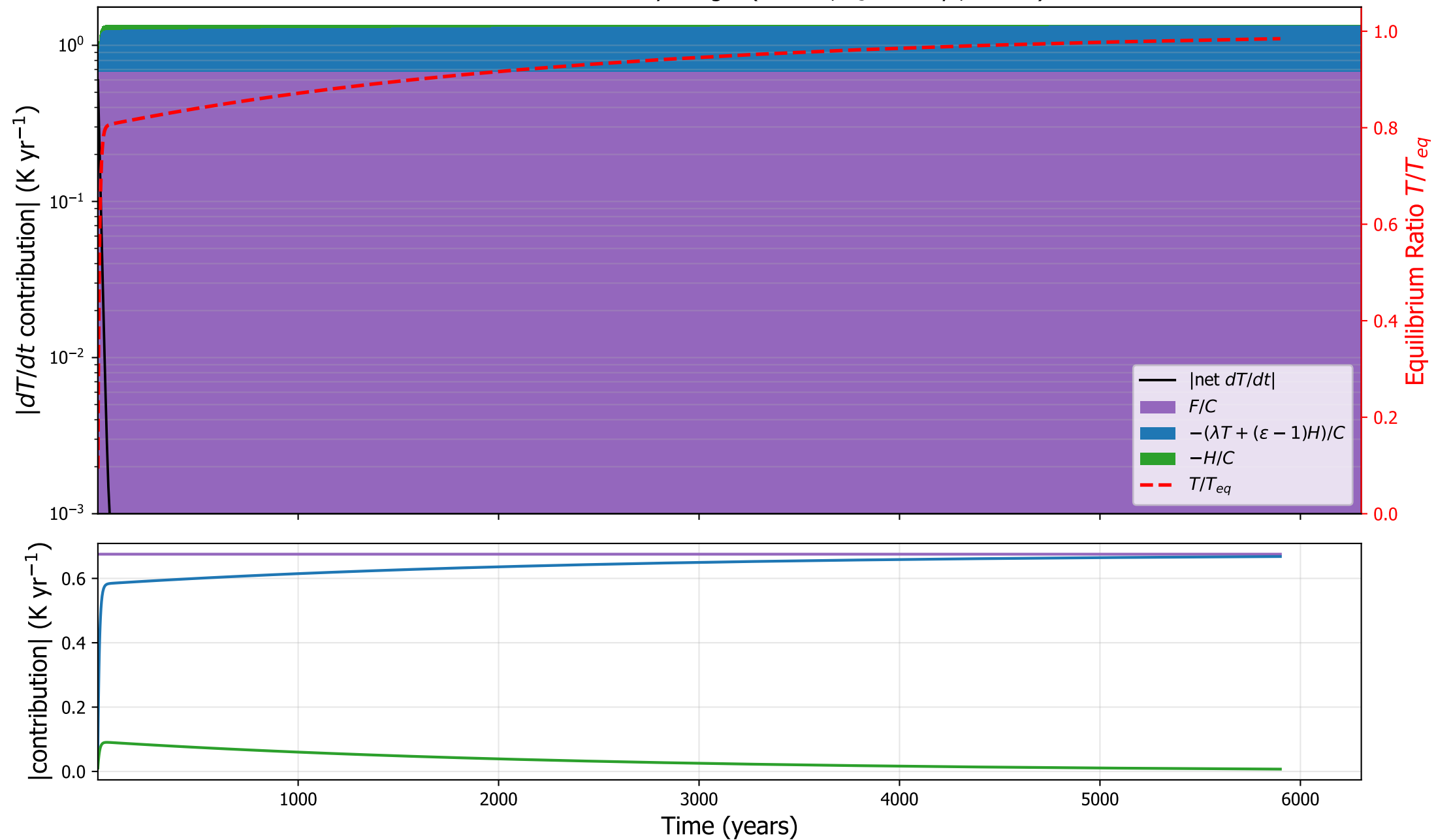
CESM1: surface tendency budget ( \varepsilon=1.44 , \tau_s=2315 yr, C=8.6 )
