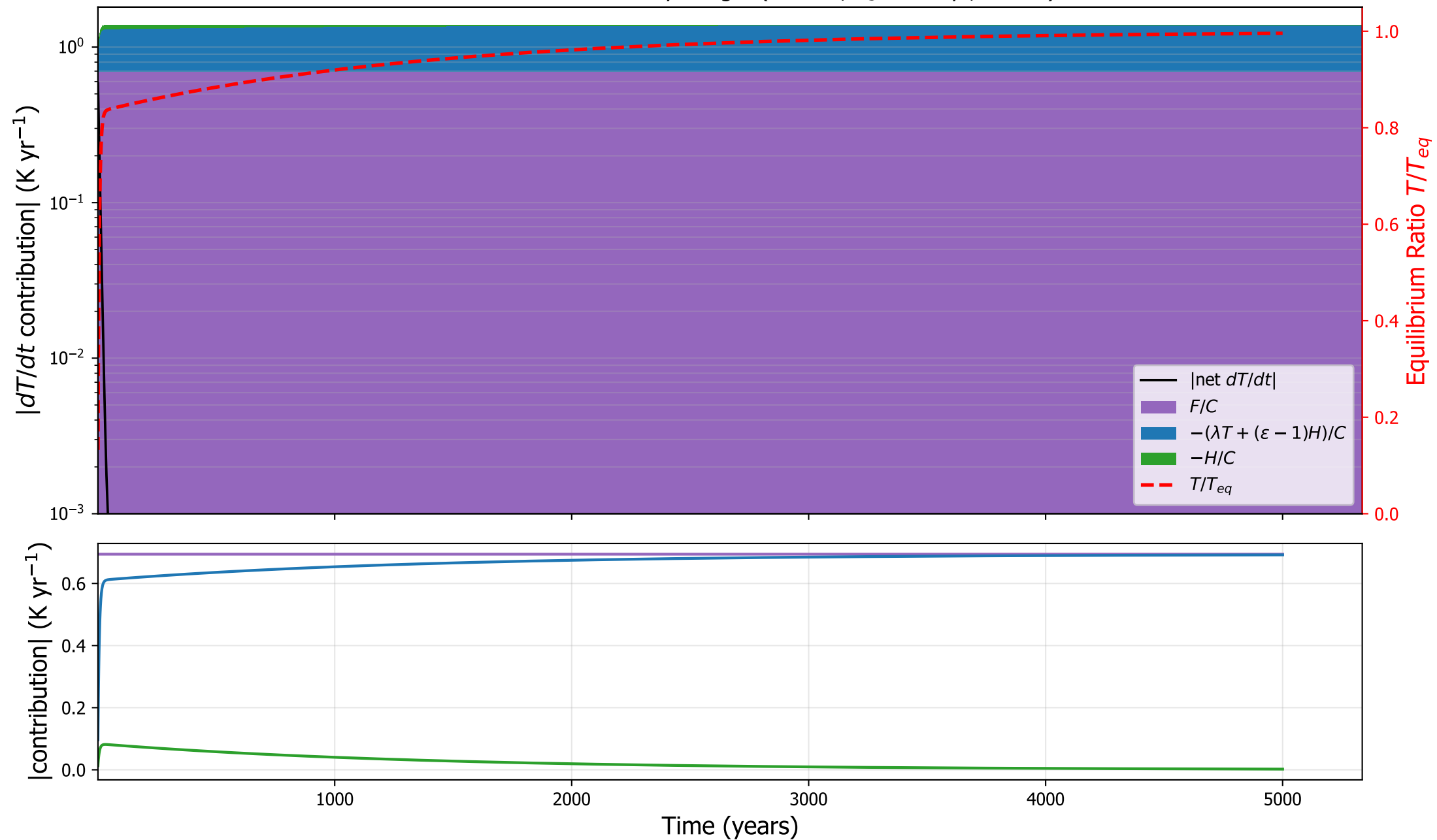
GISSE2R: surface tendency budget ( \varepsilon=1.38 , \tau_s=1363 yr, C=8.7 )
