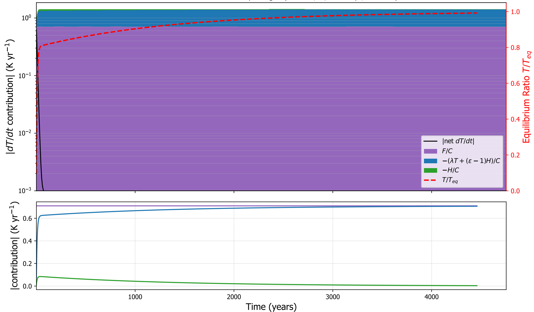
MPIESM11: surface tendency budget ( \varepsilon=1.60 , \tau_s=1385 yr, C=11.2 )
