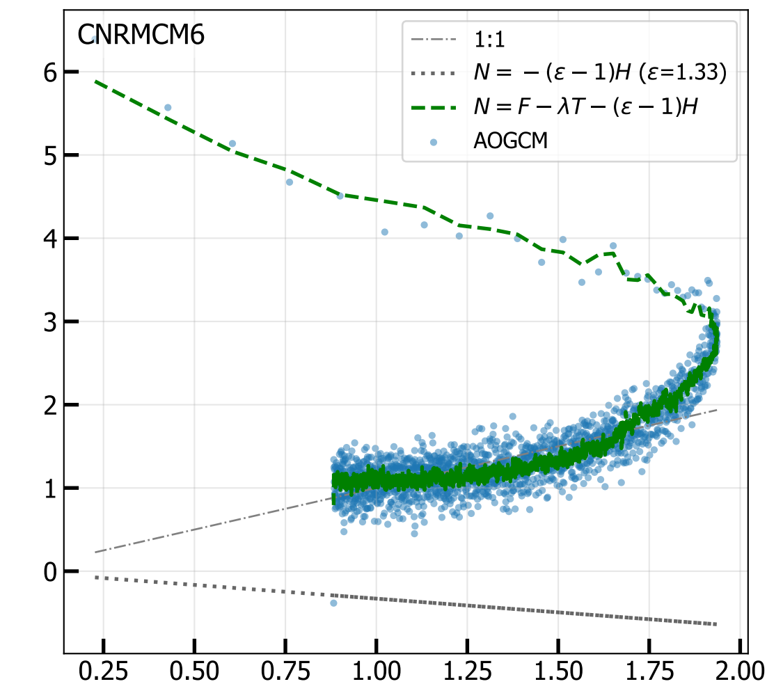
4xCO 2 Net TOA vs Ocean Heat Uptake H (radiative fit, iter 3)
