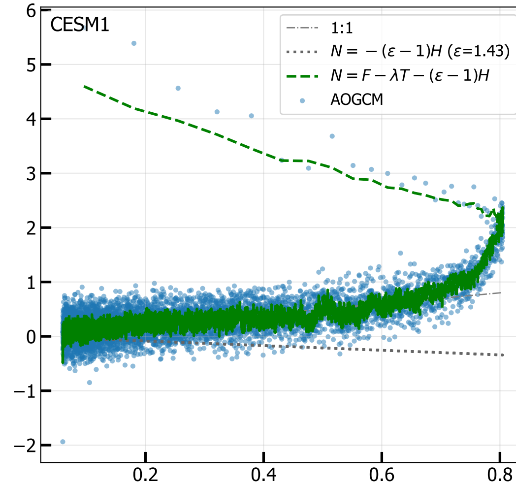
4xCO 2 Net TOA vs Ocean Heat Uptake H (radiative fit, iter 3)
